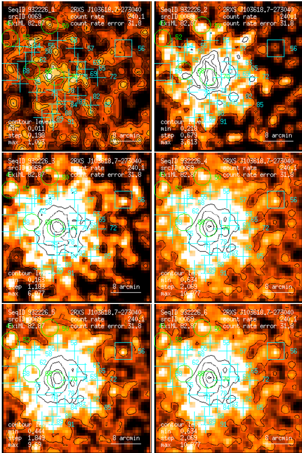
Figure 69: RASS 932226: detection 0069: band rate images, Gaussian filter: (1) PSPC channels 11 – 41, (2) 52 – 90, (3) 91 – 201, (4) 11 – 235, (5) 52 – 201, (6) 11 – 201. Broad band rates in counts/ks. Band rate contour levels in counts/ks/arcmin 2 .
