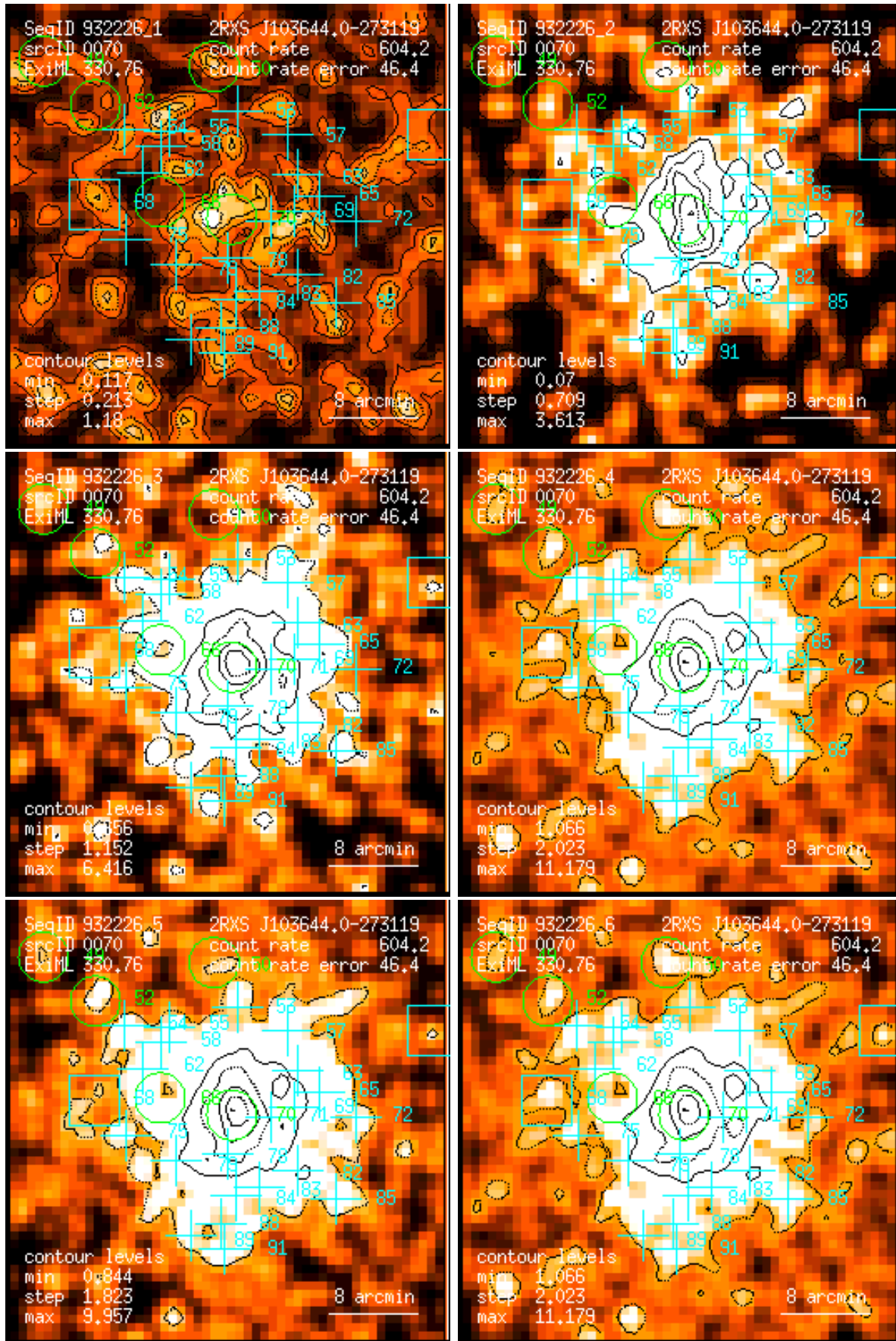
Figure 70: RASS 932226: detection 0070: band rate images, Gaussian filter: (1) PSPC channels 11 – 41, (2) 52 – 90, (3) 91 – 201, (4) 11 – 235, (5) 52 – 201, (6) 11 – 201. Broad band rates in counts/ks. Band rate contour levels in counts/ks/arcmin 2 .
