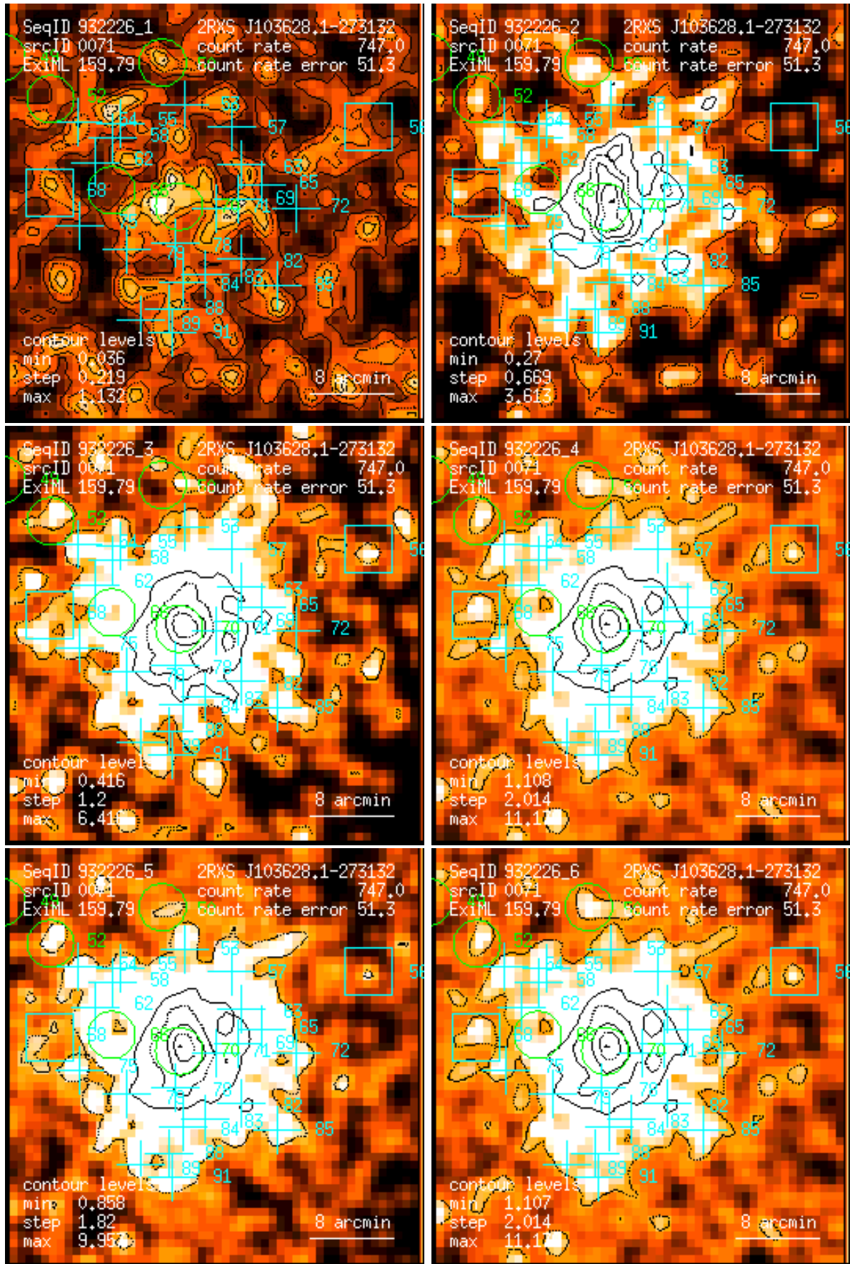
Figure 71: RASS 932226: detection 0071: band rate images, Gaussian filter: (1) PSPC channels 11 – 41, (2) 52 – 90, (3) 91 – 201, (4) 11 – 235, (5) 52 – 201, (6) 11 – 201. Broad band rates in counts/ks. Band rate contour levels in counts/ks/arcmin 2 .
