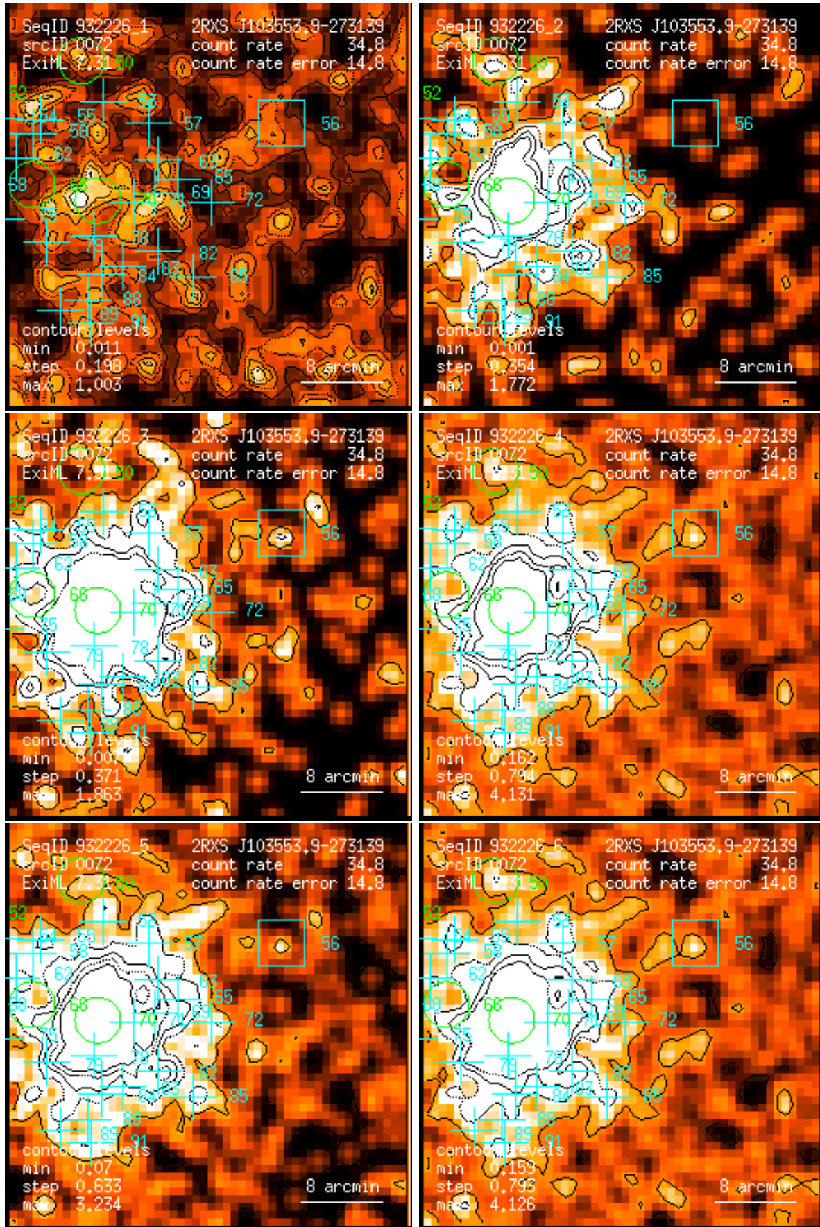
Figure 72: RASS 932226: detection 0072: band rate images, Gaussian filter: (1) PSPC channels 11 – 41, (2) 52 – 90, (3) 91 – 201, (4) 11 – 235, (5) 52 – 201, (6) 11 – 201. Broad band rates in counts/ks. Band rate contour levels in counts/ks/arcmin 2 .
