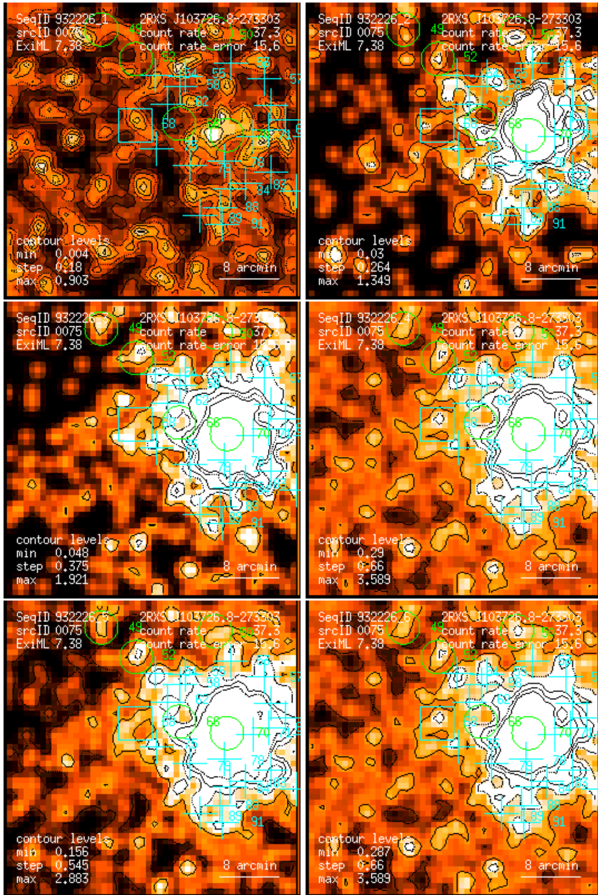
Figure 75: RASS 932226: detection 0075: band rate images, Gaussian filter: (1) PSPC channels 11 – 41, (2) 52 – 90, (3) 91 – 201, (4) 11 – 235, (5) 52 – 201, (6) 11 – 201. Broad band rates in counts/ks. Band rate contour levels in counts/ks/arcmin 2 .
