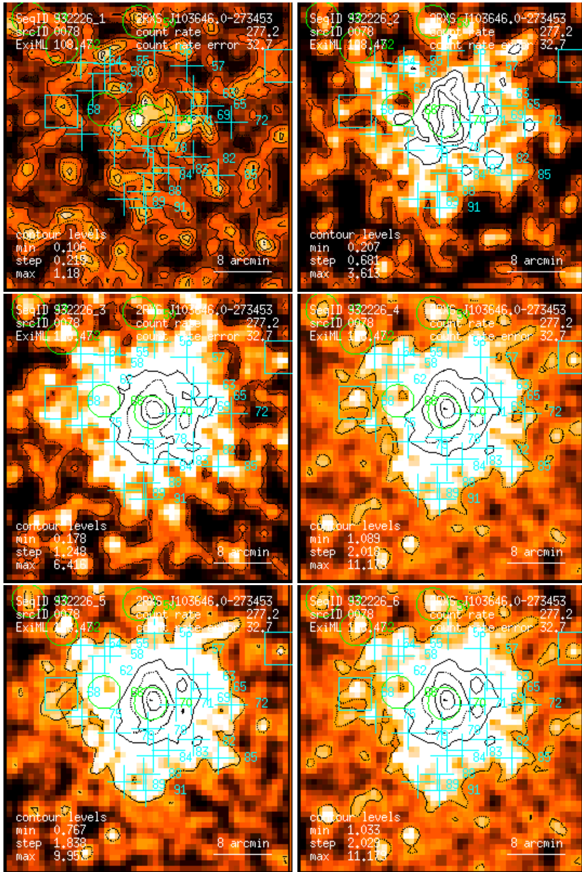
Figure 78: RASS 932226: detection 0078: band rate images, Gaussian filter: (1) PSPC channels 11 – 41, (2) 52 – 90, (3) 91 – 201, (4) 11 – 235, (5) 52 – 201, (6) 11 – 201. Broad band rates in counts/ks. Band rate contour levels in counts/ks/arcmin 2 .
