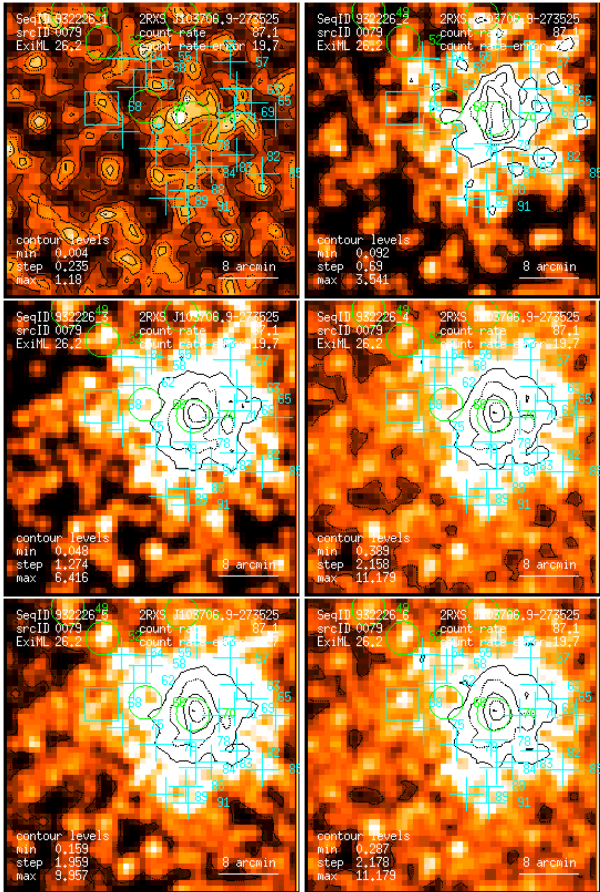
Figure 79: RASS 932226: detection 0079: band rate images, Gaussian filter: (1) PSPC channels 11 – 41, (2) 52 – 90, (3) 91 – 201, (4) 11 – 235, (5) 52 – 201, (6) 11 – 201. Broad band rates in counts/ks. Band rate contour levels in counts/ks/arcmin 2 .
