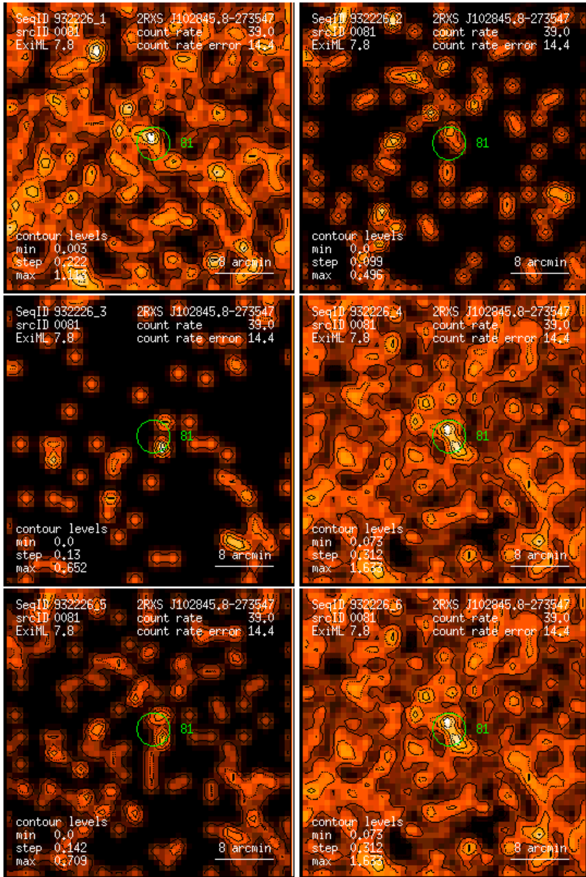
Figure 81: RASS 932226: detection 0081: band rate images, Gaussian filter: (1) PSPC channels 11 – 41, (2) 52 – 90, (3) 91 – 201, (4) 11 – 235, (5) 52 – 201, (6) 11 – 201. Broad band rates in counts/ks. Band rate contour levels in counts/ks/arcmin 2 .
