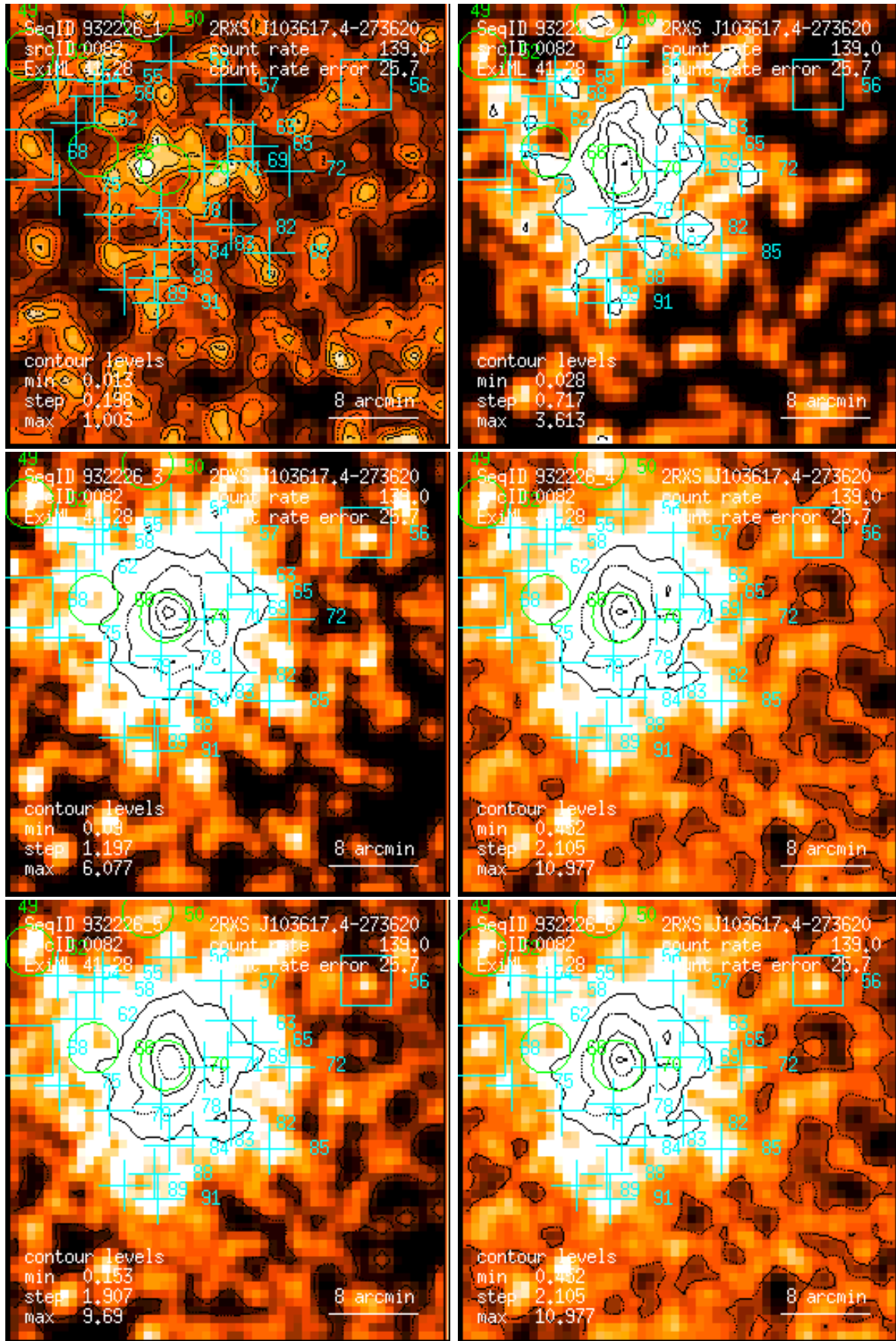
Figure 82: RASS 932226: detection 0082: band rate images, Gaussian filter: (1) PSPC channels 11 – 41, (2) 52 – 90, (3) 91 – 201, (4) 11 – 235, (5) 52 – 201, (6) 11 – 201. Broad band rates in counts/ks. Band rate contour levels in counts/ks/arcmin 2 .
