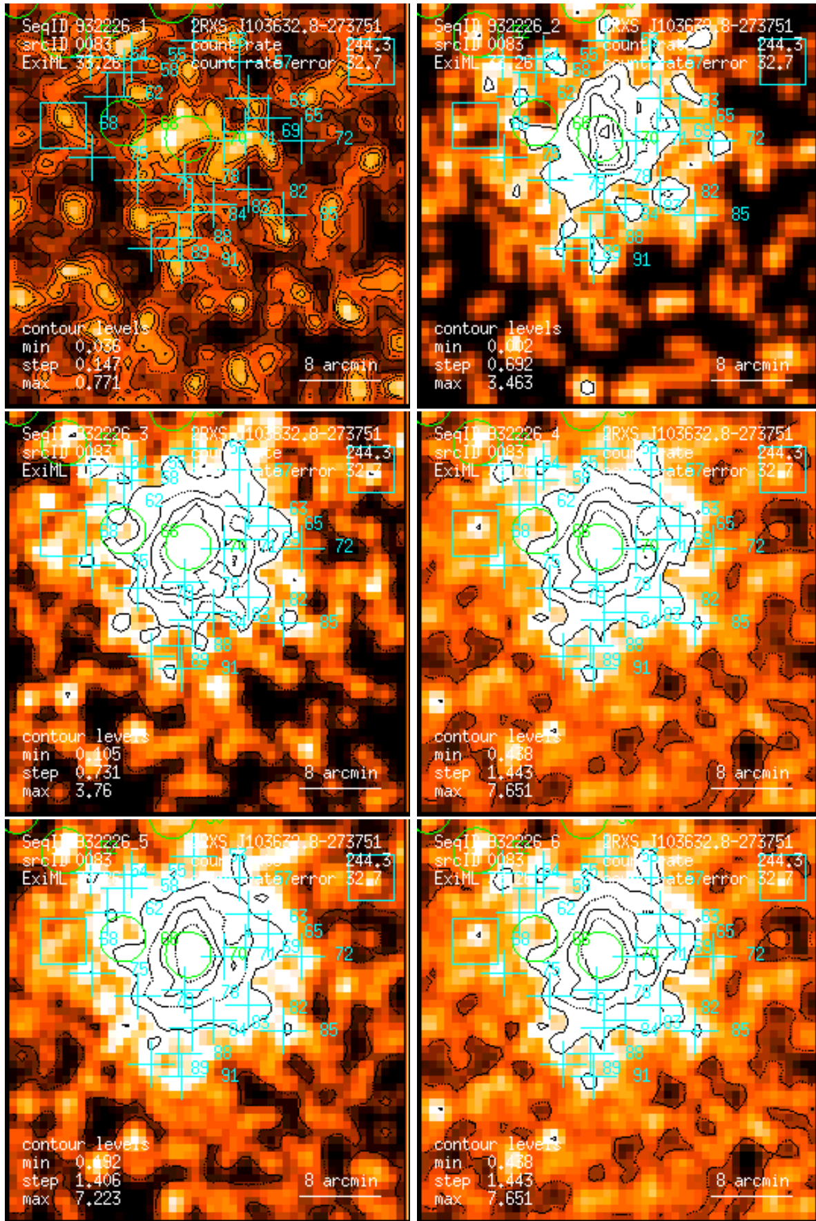
Figure 83: RASS 932226: detection 0083: band rate images, Gaussian filter: (1) PSPC channels 11 – 41, (2) 52 – 90, (3) 91 – 201, (4) 11 – 235, (5) 52 – 201, (6) 11 – 201. Broad band rates in counts/ks. Band rate contour levels in counts/ks/arcmin 2 .
