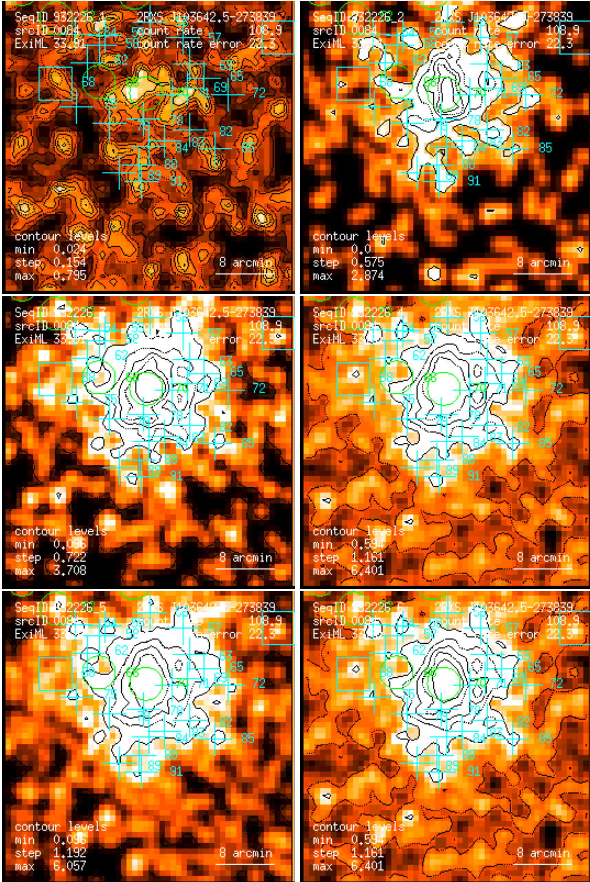
Figure 84: RASS 932226: detection 0084: band rate images, Gaussian filter: (1) PSPC channels 11 – 41, (2) 52 – 90, (3) 91 – 201, (4) 11 – 235, (5) 52 – 201, (6) 11 – 201. Broad band rates in counts/ks. Band rate contour levels in counts/ks/arcmin 2 .
