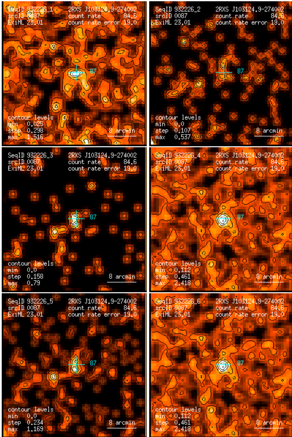
Figure 87: RASS 932226: detection 0087: band rate images, Gaussian filter: (1) PSPC channels 11 – 41, (2) 52 – 90, (3) 91 – 201, (4) 11 – 235, (5) 52 – 201, (6) 11 – 201. Broad band rates in counts/ks. Band rate contour levels in counts/ks/arcmin 2 .
