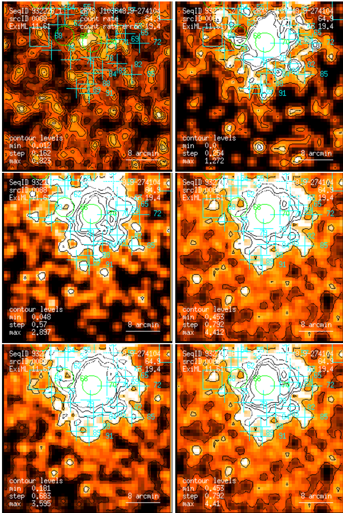
Figure 88: RASS 932226: detection 0088: band rate images, Gaussian filter: (1) PSPC channels 11 – 41, (2) 52 – 90, (3) 91 – 201, (4) 11 – 235, (5) 52 – 201, (6) 11 – 201. Broad band rates in counts/ks. Band rate contour levels in counts/ks/arcmin 2 .
