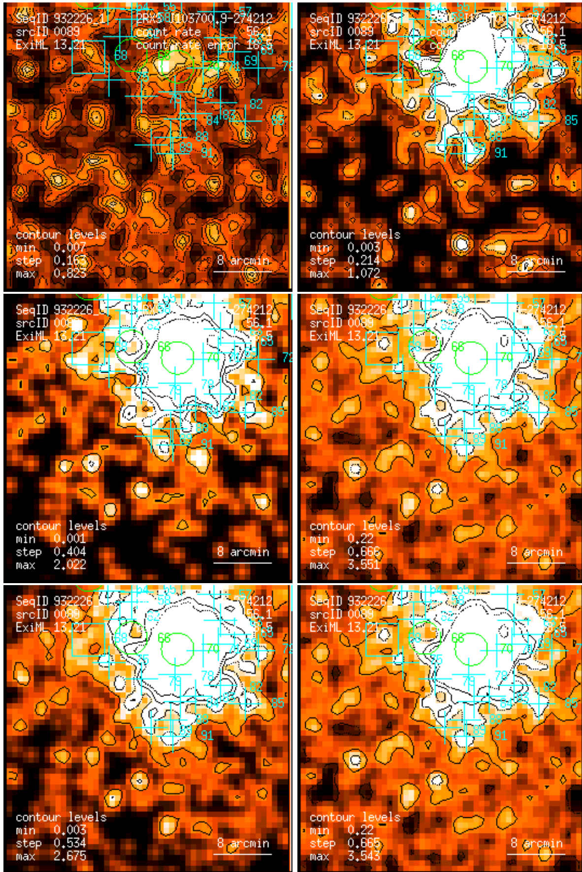
Figure 89: RASS 932226: detection 0089: band rate images, Gaussian filter: (1) PSPC channels 11 – 41, (2) 52 – 90, (3) 91 – 201, (4) 11 – 235, (5) 52 – 201, (6) 11 – 201. Broad band rates in counts/ks. Band rate contour levels in counts/ks/arcmin 2 .
