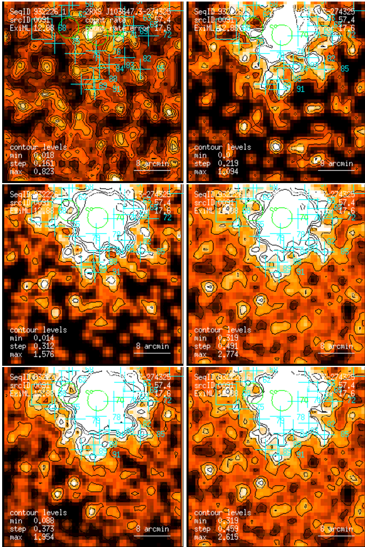
Figure 91: RASS 932226: detection 0091: band rate images, Gaussian filter: (1) PSPC channels 11 – 41, (2) 52 – 90, (3) 91 – 201, (4) 11 – 235, (5) 52 – 201, (6) 11 – 201. Broad band rates in counts/ks. Band rate contour levels in counts/ks/arcmin 2 .
