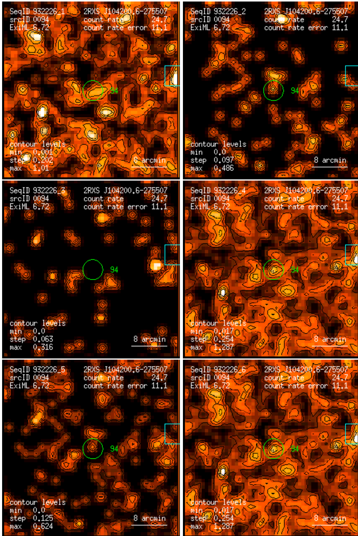
Figure 94: RASS 932226: detection 0094: band rate images, Gaussian filter: (1) PSPC channels 11 – 41, (2) 52 – 90, (3) 91 – 201, (4) 11 – 235, (5) 52 – 201, (6) 11 – 201. Broad band rates in counts/ks. Band rate contour levels in counts/ks/arcmin 2 .
