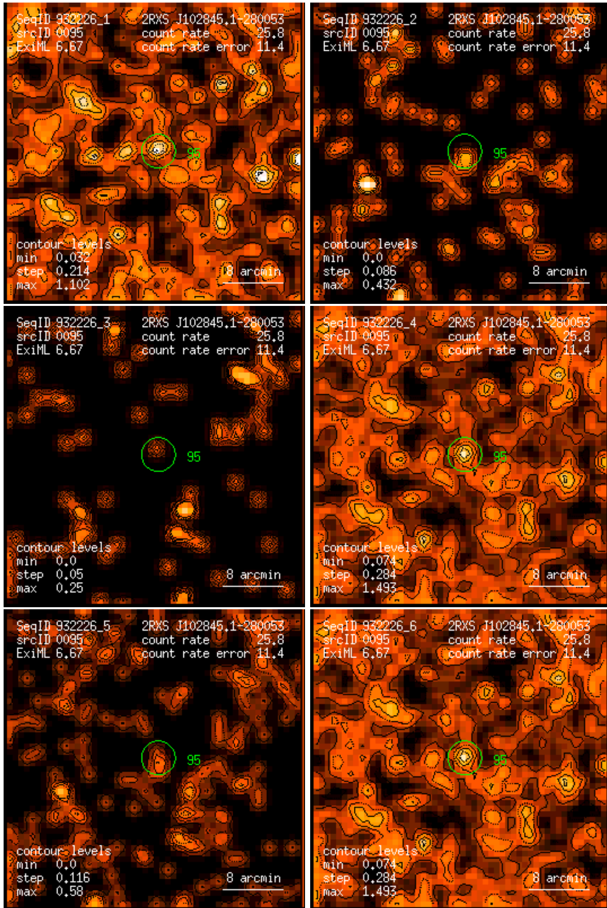
Figure 95: RASS 932226: detection 0095: band rate images, Gaussian filter: (1) PSPC channels 11 – 41, (2) 52 – 90, (3) 91 – 201, (4) 11 – 235, (5) 52 – 201, (6) 11 – 201. Broad band rates in counts/ks. Band rate contour levels in counts/ks/arcmin 2 .
