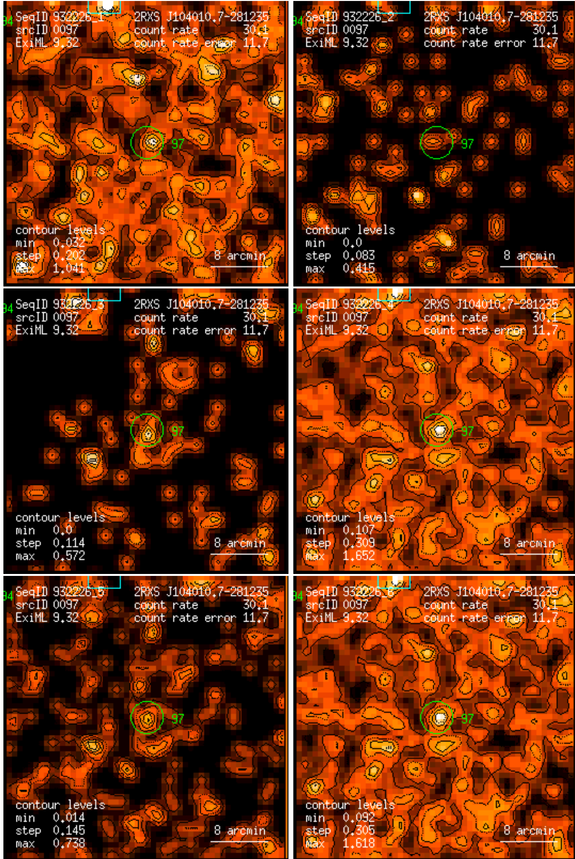
Figure 97: RASS 932226: detection 0097: band rate images, Gaussian filter: (1) PSPC channels 11 – 41, (2) 52 – 90, (3) 91 – 201, (4) 11 – 235, (5) 52 – 201, (6) 11 – 201. Broad band rates in counts/ks. Band rate contour levels in counts/ks/arcmin 2 .
