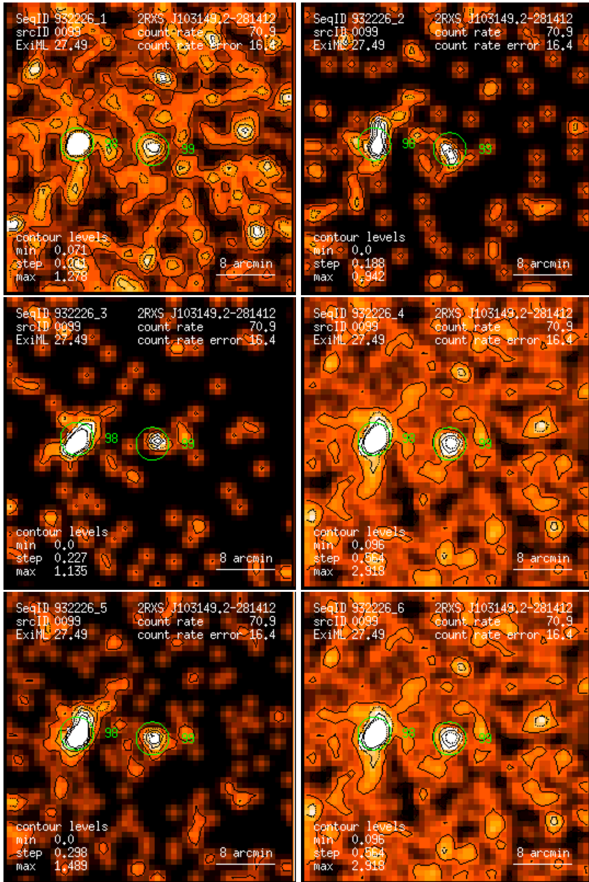
Figure 99: RASS 932226: detection 0099: band rate images, Gaussian filter: (1) PSPC channels 11 – 41, (2) 52 – 90, (3) 91 – 201, (4) 11 – 235, (5) 52 – 201, (6) 11 – 201. Broad band rates in counts/ks. Band rate contour levels in counts/ks/arcmin 2 .
