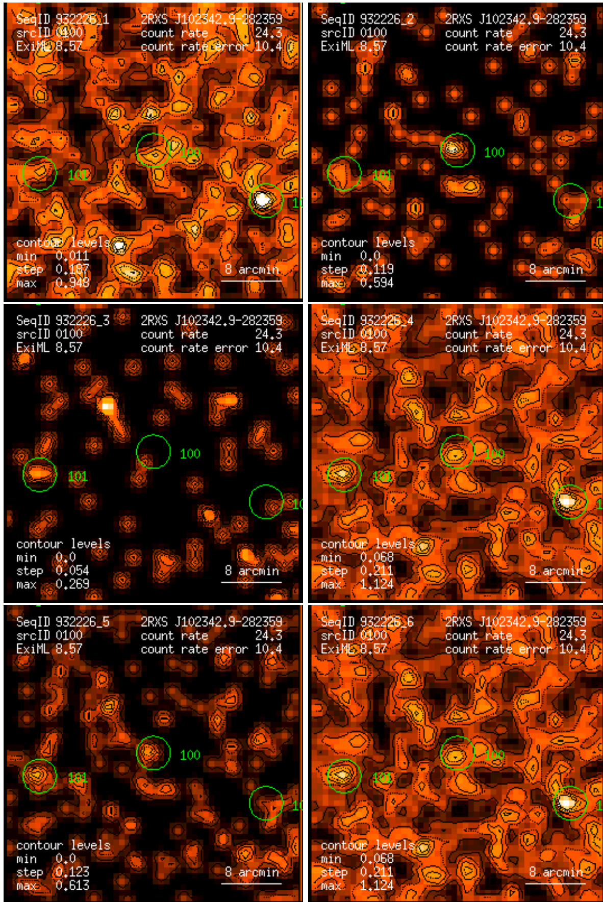
Figure 100: RASS 932226: detection 0100: band rate images, Gaussian filter: (1) PSPC channels 11 – 41, (2) 52 – 90, (3) 91 – 201, (4) 11 – 235, (5) 52 – 201, (6) 11 – 201. Broad band rates in counts/ks. Band rate contour levels in counts/ks/arcmin 2 .
