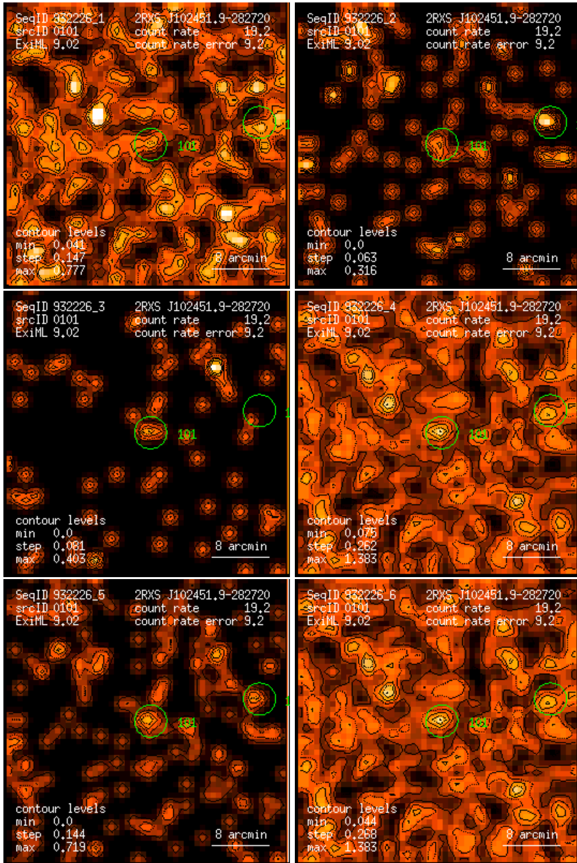
Figure 101: RASS 932226: detection 0101: band rate images, Gaussian filter: (1) PSPC channels 11 – 41, (2) 52 – 90, (3) 91 – 201, (4) 11 – 235, (5) 52 – 201, (6) 11 – 201. Broad band rates in counts/ks. Band rate contour levels in counts/ks/arcmin 2 .
