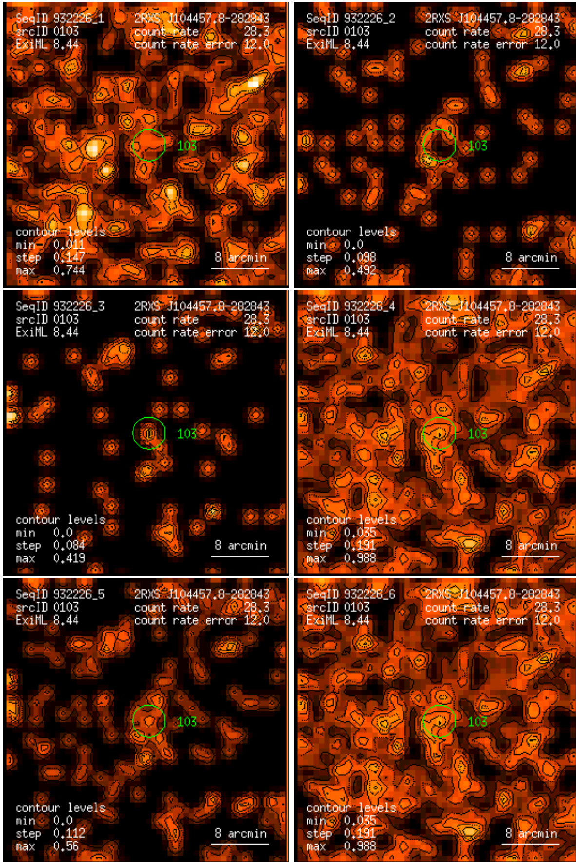
Figure 103: RASS 932226: detection 0103: band rate images, Gaussian filter: (1) PSPC channels 11 – 41, (2) 52 – 90, (3) 91 – 201, (4) 11 – 235, (5) 52 – 201, (6) 11 – 201. Broad band rates in counts/ks. Band rate contour levels in counts/ks/arcmin 2 .
