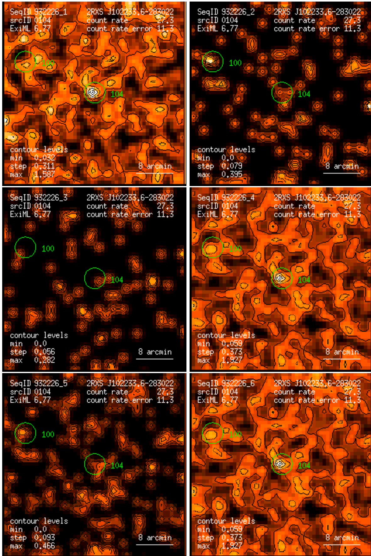
Figure 104: RASS 932226: detection 0104: band rate images, Gaussian filter: (1) PSPC channels 11 – 41, (2) 52 – 90, (3) 91 – 201, (4) 11 – 235, (5) 52 – 201, (6) 11 – 201. Broad band rates in counts/ks. Band rate contour levels in counts/ks/arcmin 2 .
