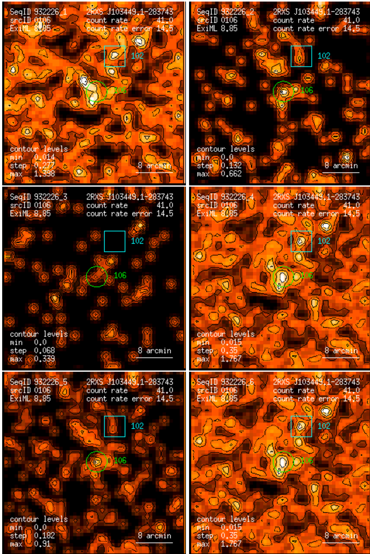
Figure 106: RASS 932226: detection 0106: band rate images, Gaussian filter: (1) PSPC channels 11 – 41, (2) 52 – 90, (3) 91 – 201, (4) 11 – 235, (5) 52 – 201, (6) 11 – 201. Broad band rates in counts/ks. Band rate contour levels in counts/ks/arcmin 2 .
