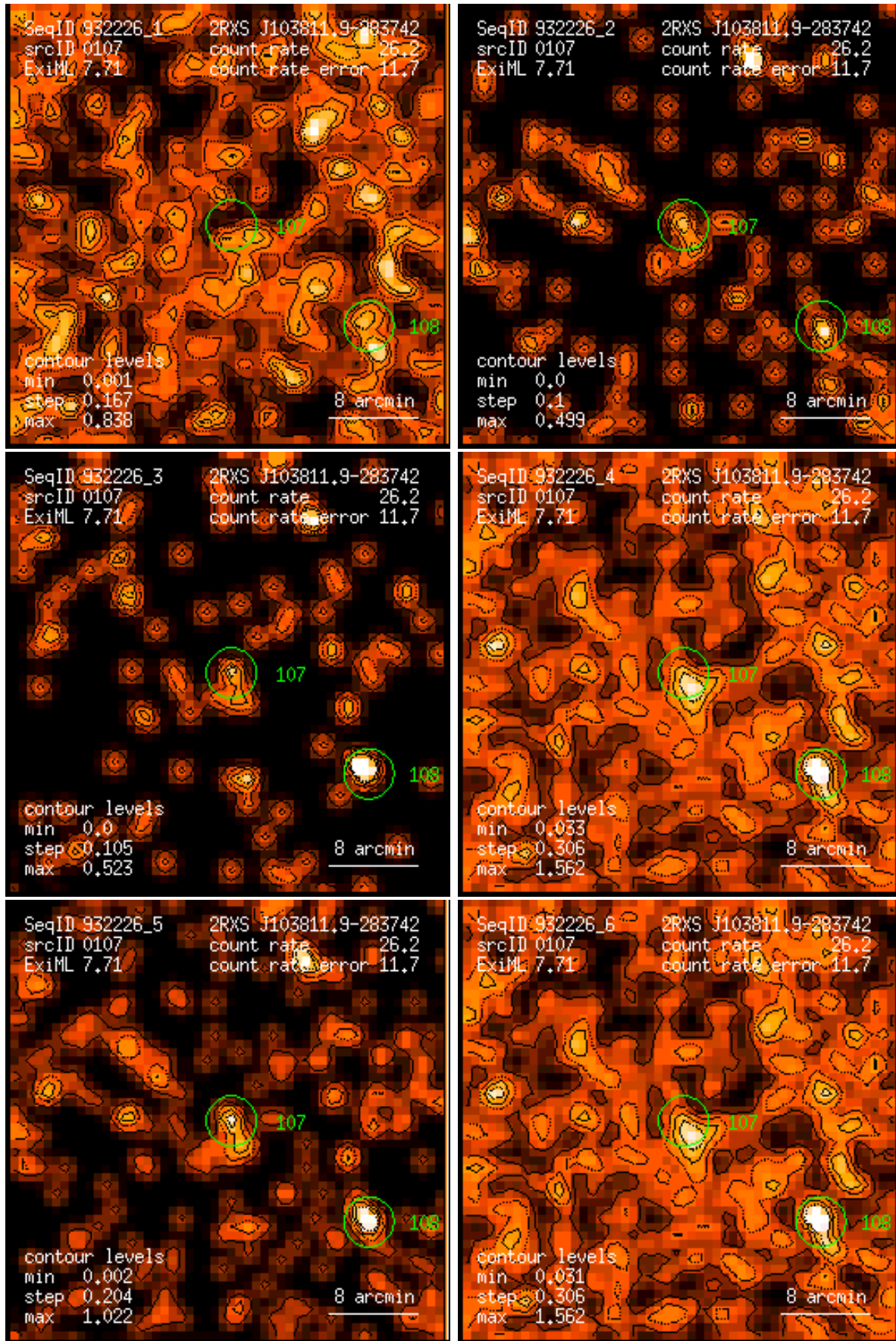
Figure 107: RASS 932226: detection 0107: band rate images, Gaussian filter: (1) PSPC channels 11 – 41, (2) 52 – 90, (3) 91 – 201, (4) 11 – 235, (5) 52 – 201, (6) 11 – 201. Broad band rates in counts/ks. Band rate contour levels in counts/ks/arcmin 2 .
