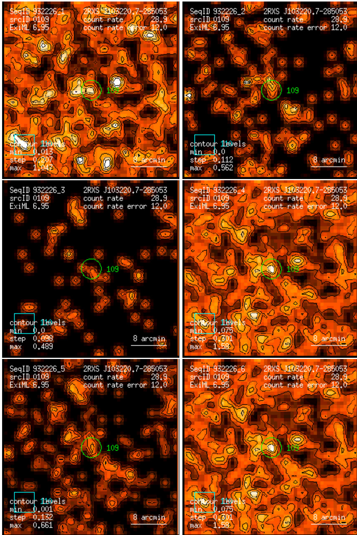
Figure 109: RASS 932226: detection 0109: band rate images, Gaussian filter: (1) PSPC channels 11 – 41, (2) 52 – 90, (3) 91 – 201, (4) 11 – 235, (5) 52 – 201, (6) 11 – 201. Broad band rates in counts/ks. Band rate contour levels in counts/ks/arcmin 2 .
