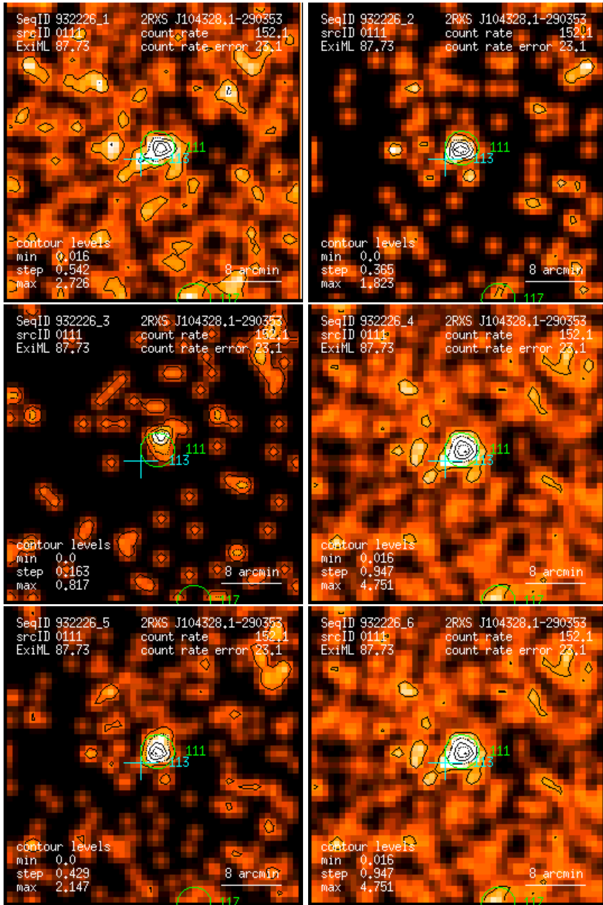
Figure 111: RASS 932226: detection 0111: band rate images, Gaussian filter: (1) PSPC channels 11 – 41, (2) 52 – 90, (3) 91 – 201, (4) 11 – 235, (5) 52 – 201, (6) 11 – 201. Broad band rates in counts/ks. Band rate contour levels in counts/ks/arcmin 2 .
