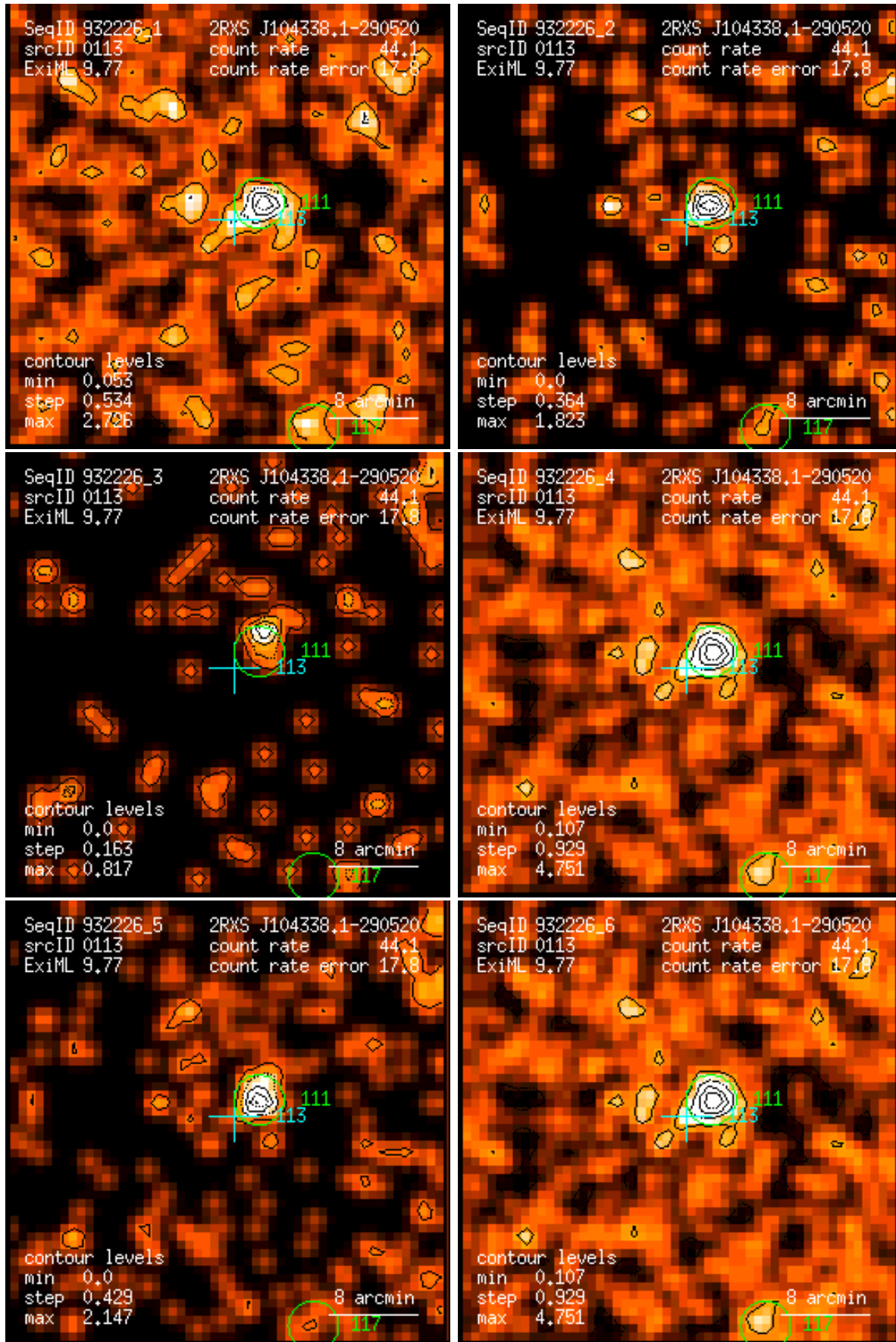
Figure 113: RASS 932226: detection 0113: band rate images, Gaussian filter: (1) PSPC channels 11 – 41, (2) 52 – 90, (3) 91 – 201, (4) 11 – 235, (5) 52 – 201, (6) 11 – 201. Broad band rates in counts/ks. Band rate contour levels in counts/ks/arcmin 2 .
