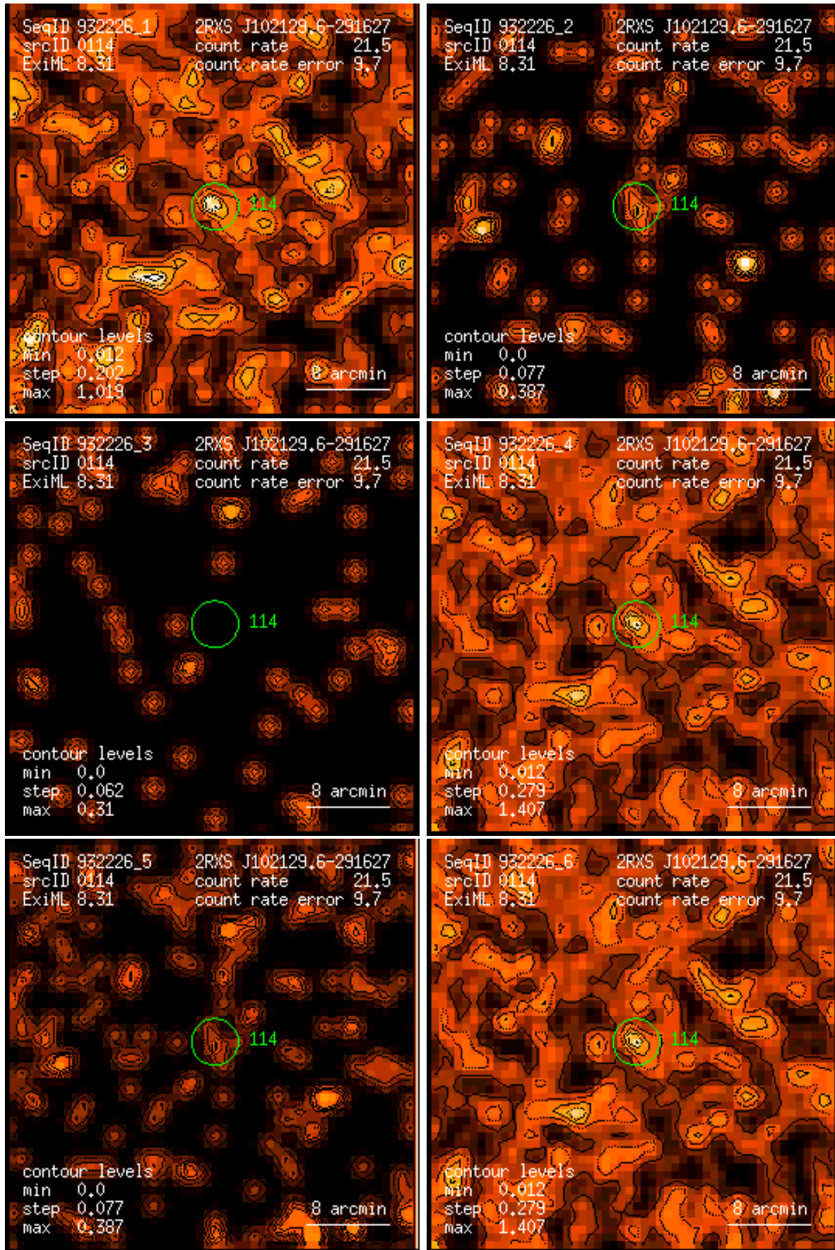
Figure 114: RASS 932226: detection 0114: band rate images, Gaussian filter: (1) PSPC channels 11 – 41, (2) 52 – 90, (3) 91 – 201, (4) 11 – 235, (5) 52 – 201, (6) 11 – 201. Broad band rates in counts/ks. Band rate contour levels in counts/ks/arcmin 2 .
