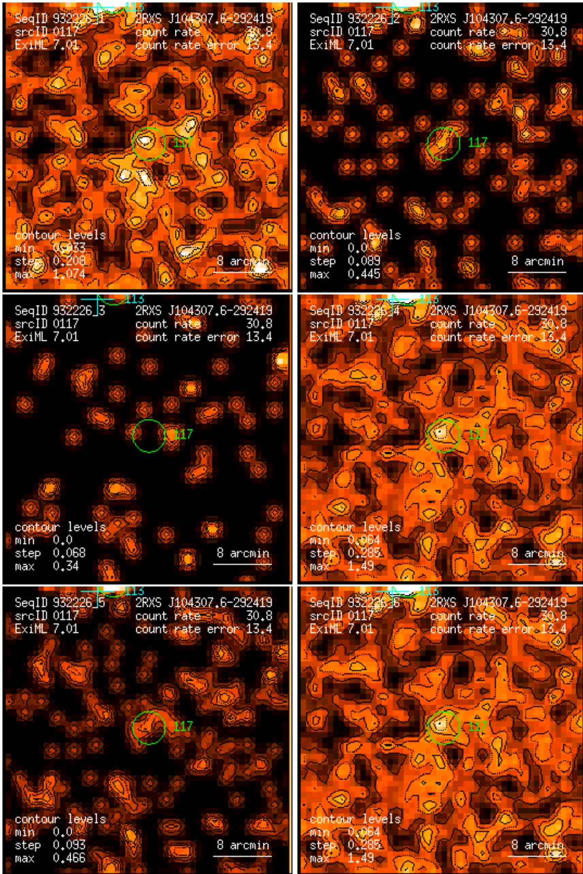
Figure 117: RASS 932226: detection 0117: band rate images, Gaussian filter: (1) PSPC channels 11 – 41, (2) 52 – 90, (3) 91 – 201, (4) 11 – 235, (5) 52 – 201, (6) 11 – 201. Broad band rates in counts/ks. Band rate contour levels in counts/ks/arcmin 2 .
