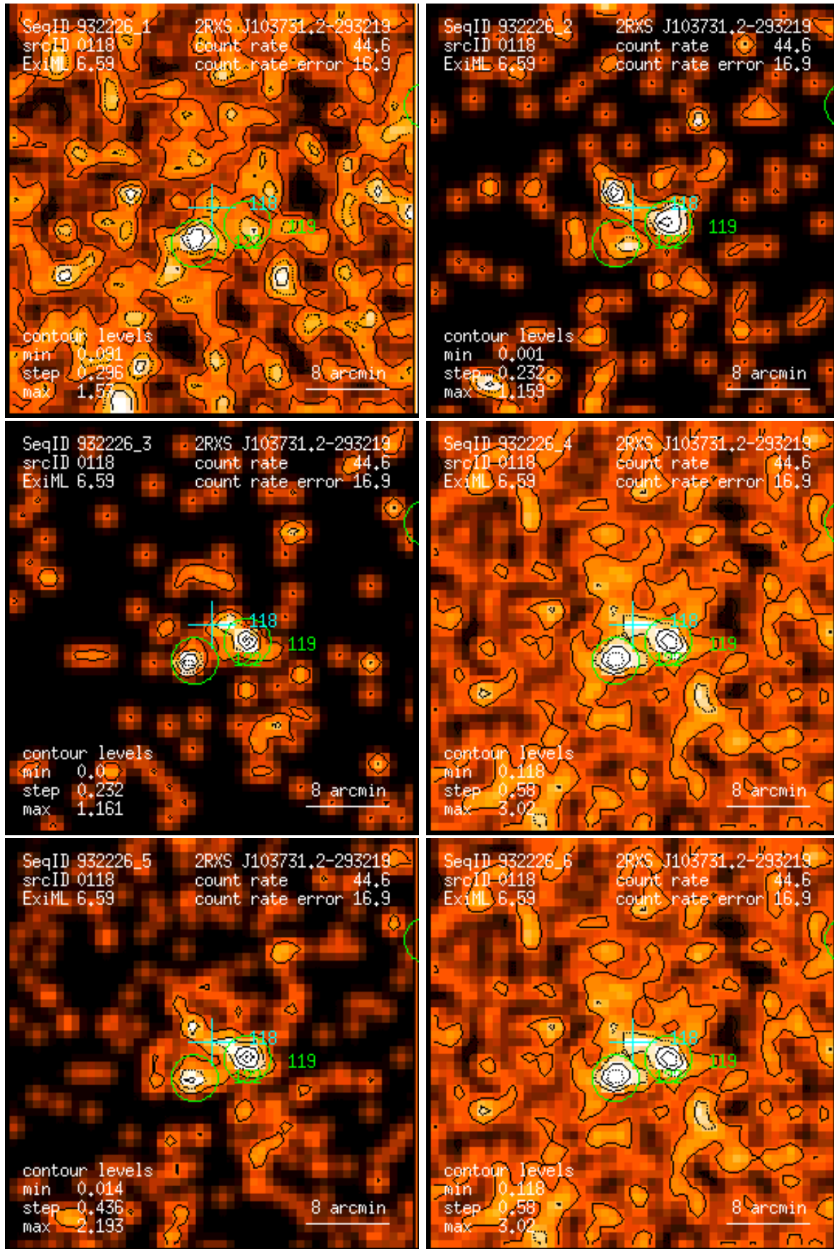
Figure 118: RASS 932226: detection 0118: band rate images, Gaussian filter: (1) PSPC channels 11 – 41, (2) 52 – 90, (3) 91 – 201, (4) 11 – 235, (5) 52 – 201, (6) 11 – 201. Broad band rates in counts/ks. Band rate contour levels in counts/ks/arcmin 2 .
