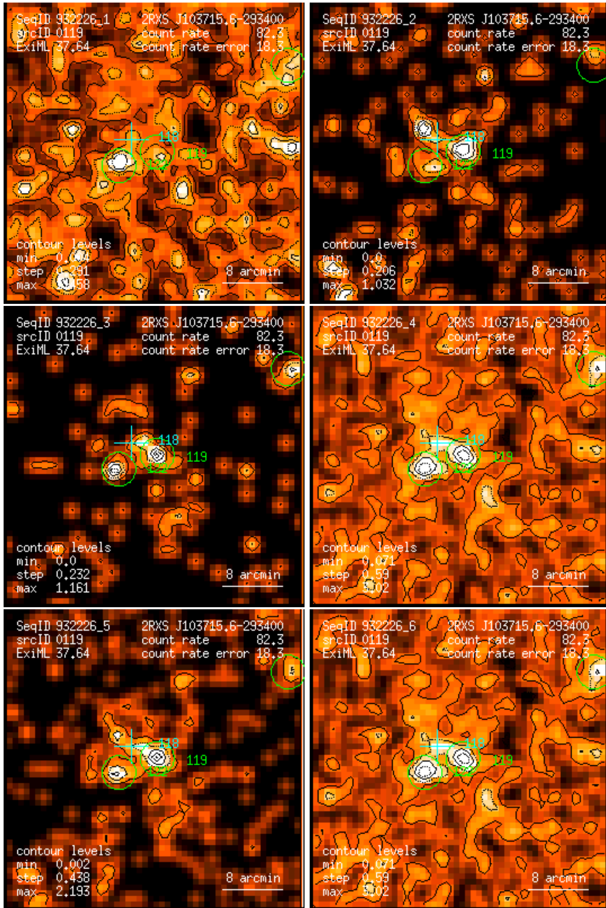
Figure 119: RASS 932226: detection 0119: band rate images, Gaussian filter: (1) PSPC channels 11 – 41, (2) 52 – 90, (3) 91 – 201, (4) 11 – 235, (5) 52 – 201, (6) 11 – 201. Broad band rates in counts/ks. Band rate contour levels in counts/ks/arcmin 2 .
