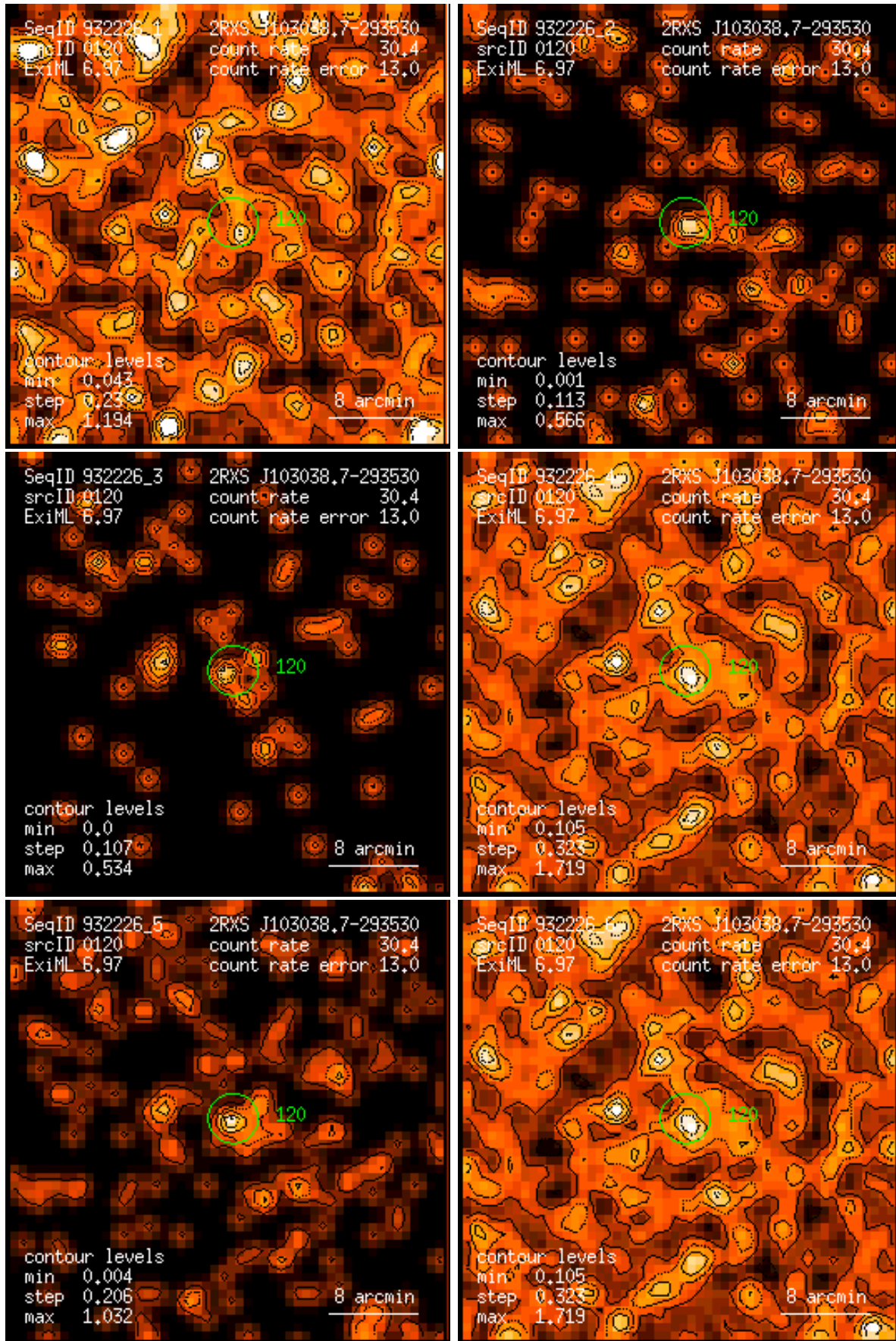
Figure 120: RASS 932226: detection 0120: band rate images, Gaussian filter: (1) PSPC channels 11 – 41, (2) 52 – 90, (3) 91 – 201, (4) 11 – 235, (5) 52 – 201, (6) 11 – 201. Broad band rates in counts/ks. Band rate contour levels in counts/ks/arcmin 2 .
