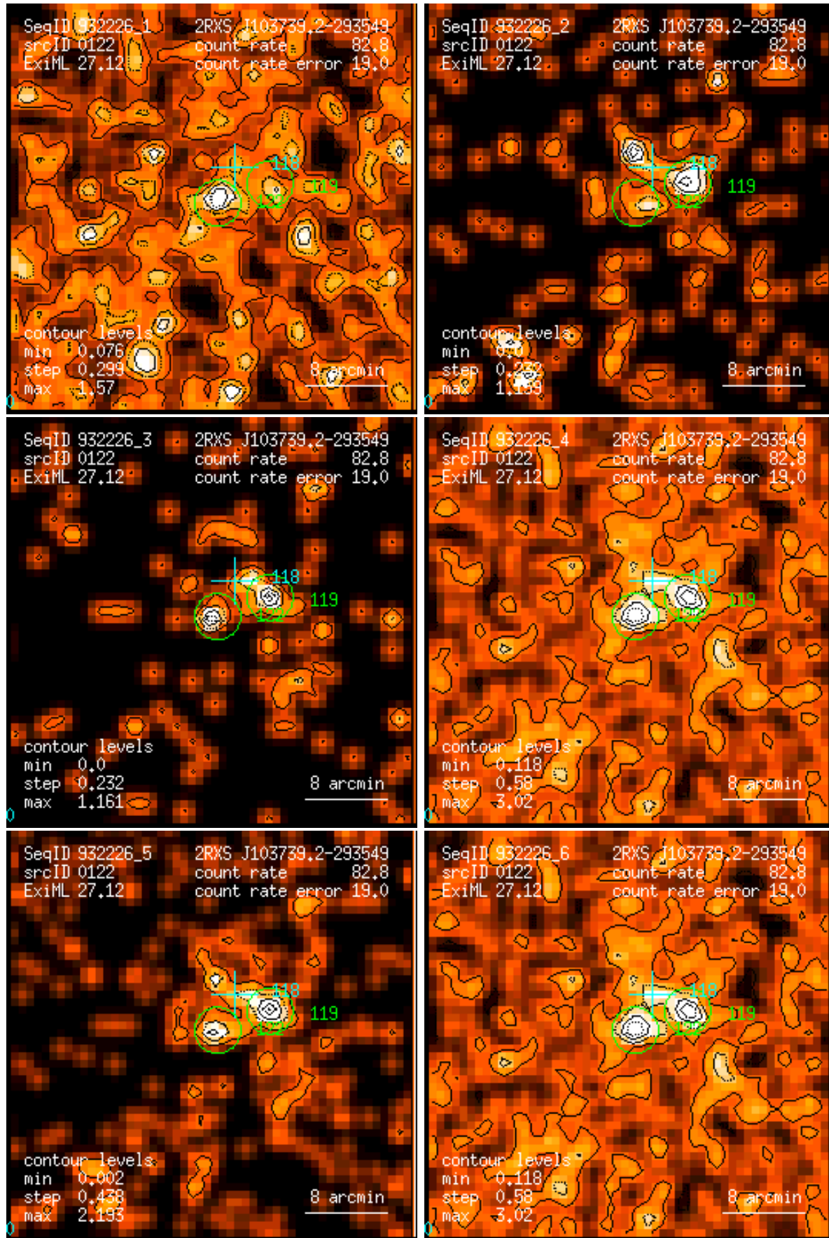
Figure 122: RASS 932226: detection 0122: band rate images, Gaussian filter: (1) PSPC channels 11 – 41, (2) 52 – 90, (3) 91 – 201, (4) 11 – 235, (5) 52 – 201, (6) 11 – 201. Broad band rates in counts/ks. Band rate contour levels in counts/ks/arcmin 2 .
