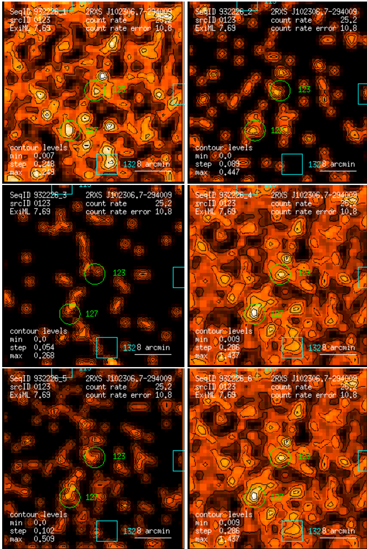
Figure 123: RASS 932226: detection 0123: band rate images, Gaussian filter: (1) PSPC channels 11 – 41, (2) 52 – 90, (3) 91 – 201, (4) 11 – 235, (5) 52 – 201, (6) 11 – 201. Broad band rates in counts/ks. Band rate contour levels in counts/ks/arcmin 2 .
