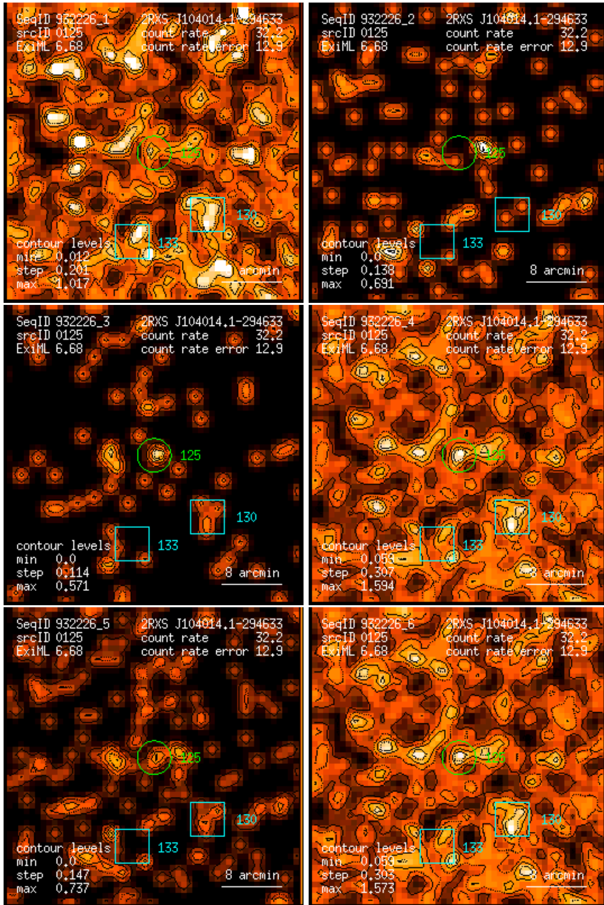
Figure 125: RASS 932226: detection 0125: band rate images, Gaussian filter: (1) PSPC channels 11 – 41, (2) 52 – 90, (3) 91 – 201, (4) 11 – 235, (5) 52 – 201, (6) 11 – 201. Broad band rates in counts/ks. Band rate contour levels in counts/ks/arcmin 2 .
