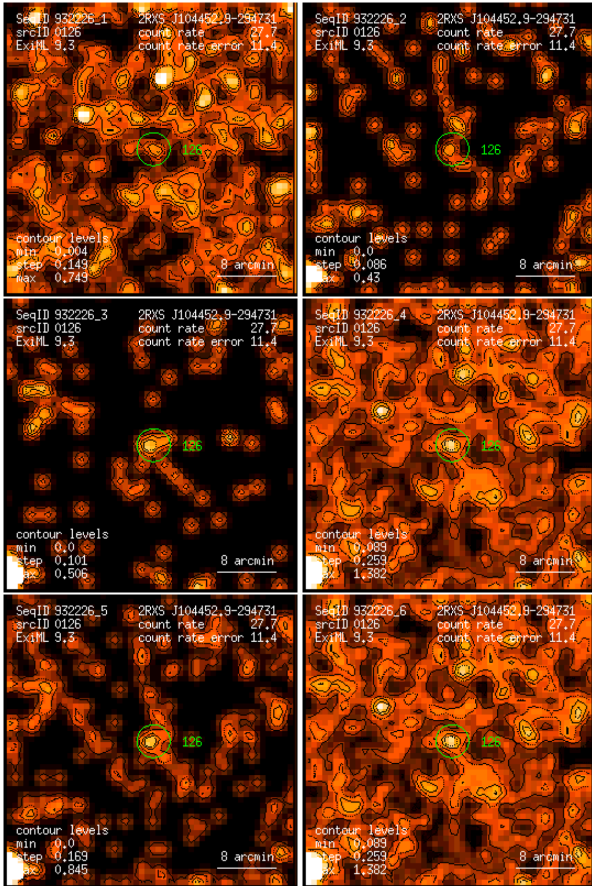
Figure 126: RASS 932226: detection 0126: band rate images, Gaussian filter: (1) PSPC channels 11 – 41, (2) 52 – 90, (3) 91 – 201, (4) 11 – 235, (5) 52 – 201, (6) 11 – 201. Broad band rates in counts/ks. Band rate contour levels in counts/ks/arcmin 2 .
