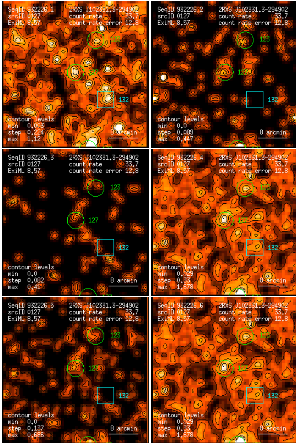
Figure 127: RASS 932226: detection 0127: band rate images, Gaussian filter: (1) PSPC channels 11 – 41, (2) 52 – 90, (3) 91 – 201, (4) 11 – 235, (5) 52 – 201, (6) 11 – 201. Broad band rates in counts/ks. Band rate contour levels in counts/ks/arcmin 2 .
