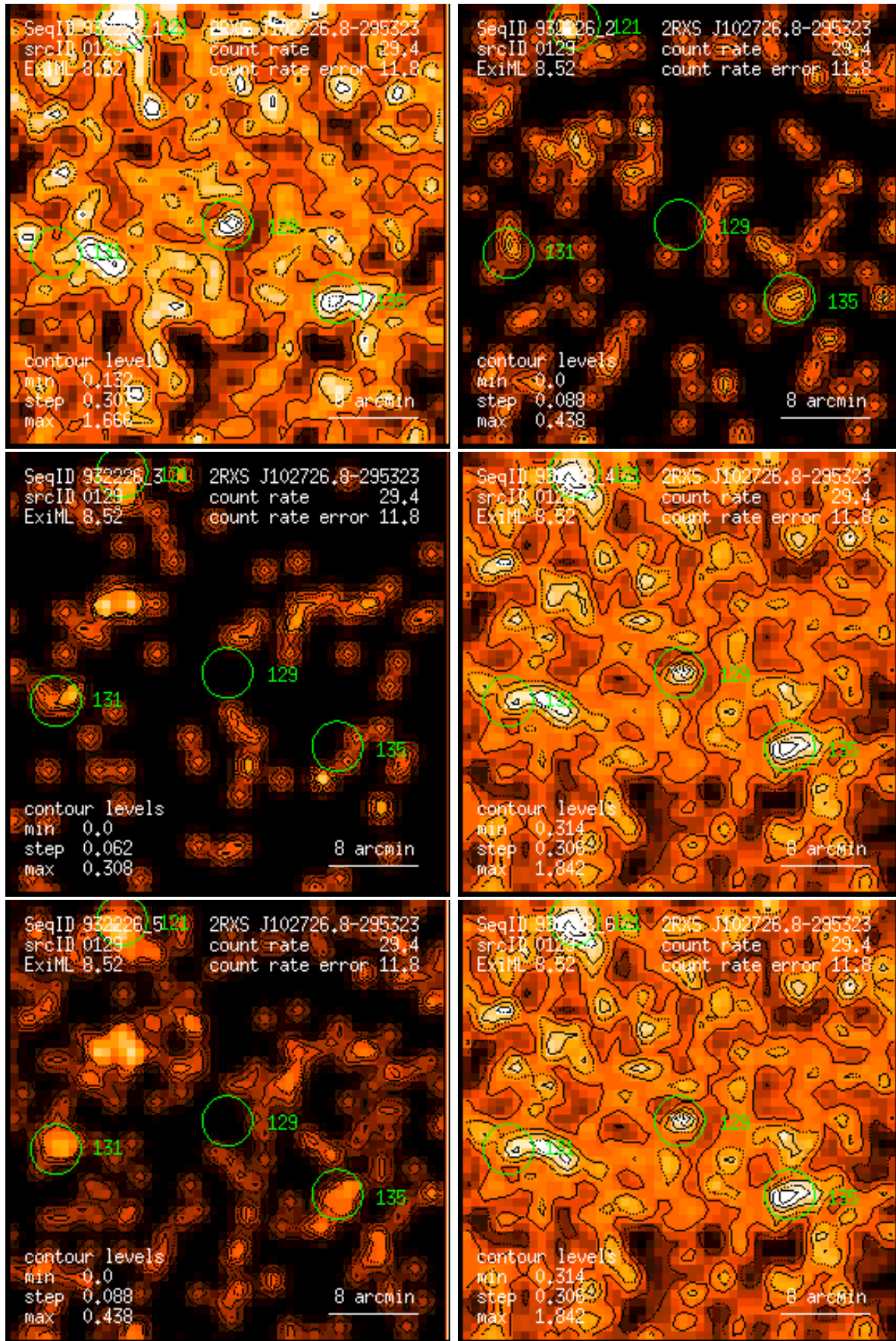
Figure 129: RASS 932226: detection 0129: band rate images, Gaussian filter: (1) PSPC channels 11 – 41, (2) 52 – 90, (3) 91 – 201, (4) 11 – 235, (5) 52 – 201, (6) 11 – 201. Broad band rates in counts/ks. Band rate contour levels in counts/ks/arcmin 2 .
