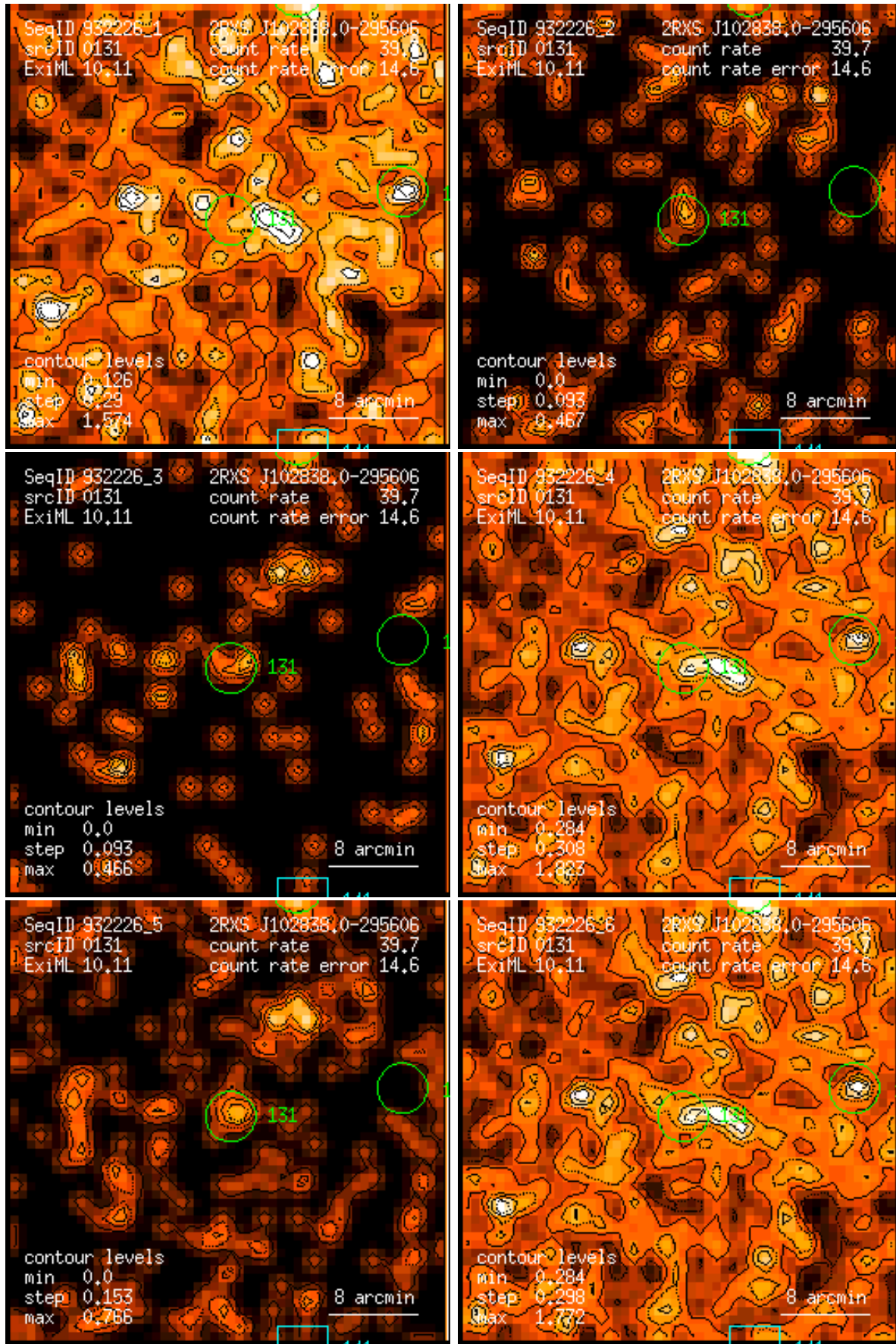
Figure 131: RASS 932226: detection 0131: band rate images, Gaussian filter: (1) PSPC channels 11 – 41, (2) 52 – 90, (3) 91 – 201, (4) 11 – 235, (5) 52 – 201, (6) 11 – 201. Broad band rates in counts/ks. Band rate contour levels in counts/ks/arcmin 2 .
