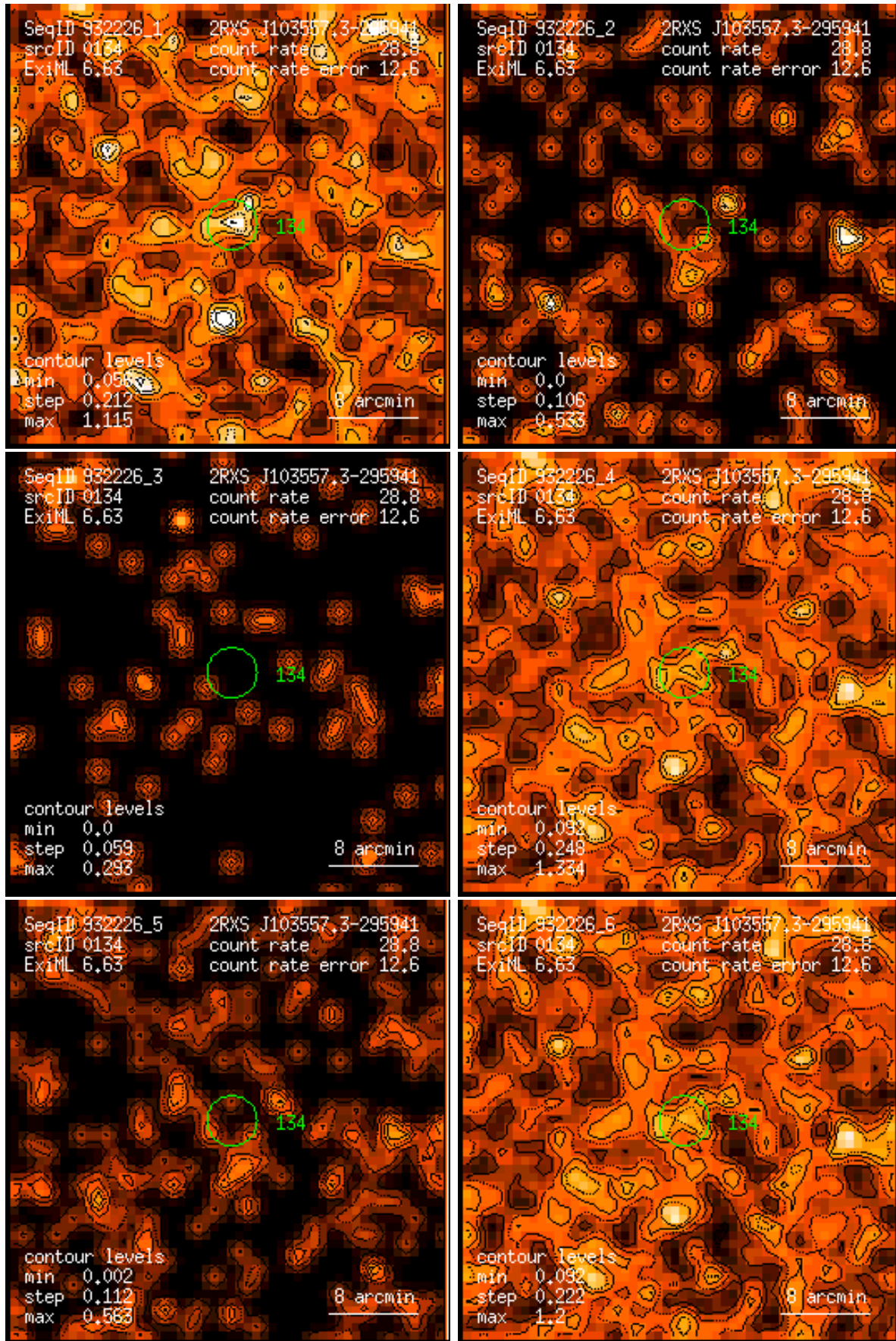
Figure 134: RASS 932226: detection 0134: band rate images, Gaussian filter: (1) PSPC channels 11 – 41, (2) 52 – 90, (3) 91 – 201, (4) 11 – 235, (5) 52 – 201, (6) 11 – 201. Broad band rates in counts/ks. Band rate contour levels in counts/ks/arcmin 2 .
