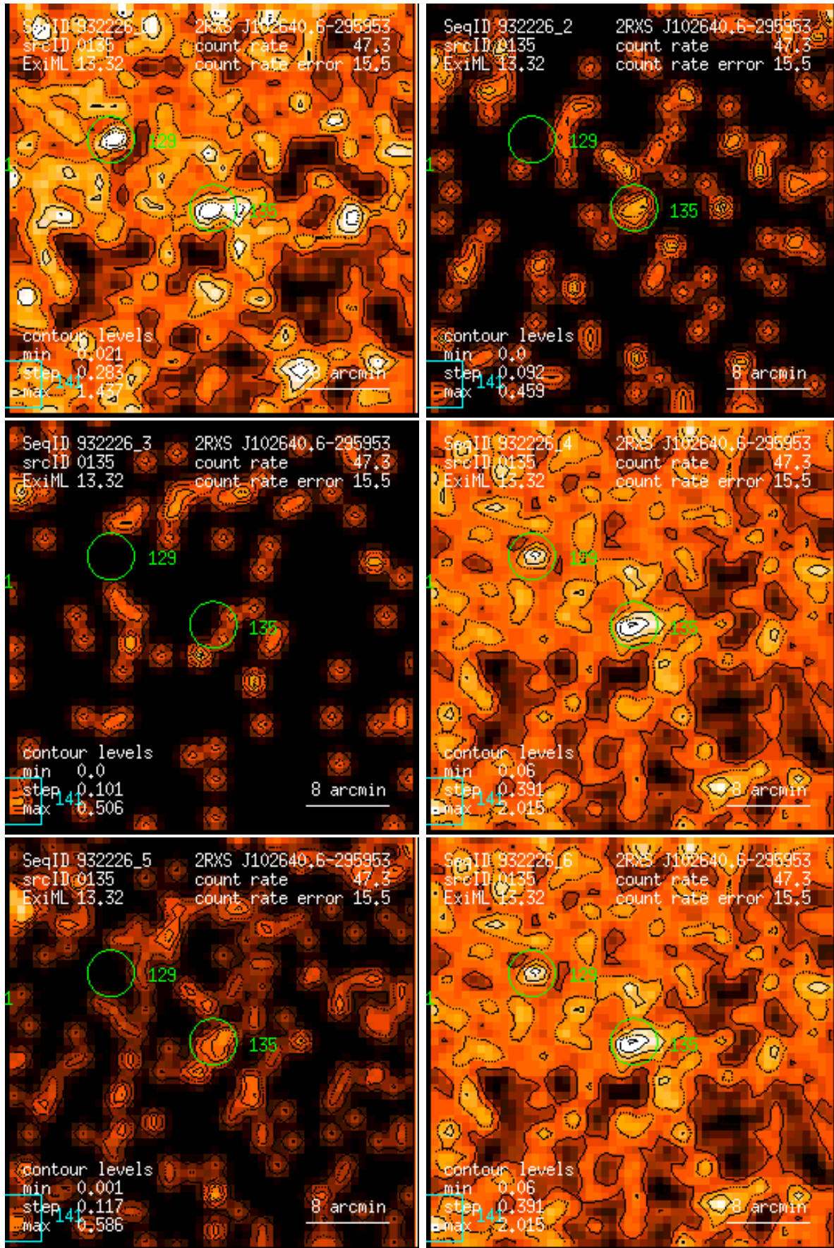
Figure 135: RASS 932226: detection 0135: band rate images, Gaussian filter: (1) PSPC channels 11 – 41, (2) 52 – 90, (3) 91 – 201, (4) 11 – 235, (5) 52 – 201, (6) 11 – 201. Broad band rates in counts/ks. Band rate contour levels in counts/ks/arcmin 2 .
