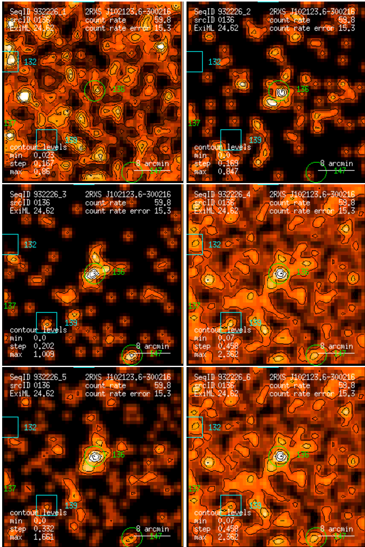
Figure 136: RASS 932226: detection 0136: band rate images, Gaussian filter: (1) PSPC channels 11 – 41, (2) 52 – 90, (3) 91 – 201, (4) 11 – 235, (5) 52 – 201, (6) 11 – 201. Broad band rates in counts/ks. Band rate contour levels in counts/ks/arcmin 2 .
