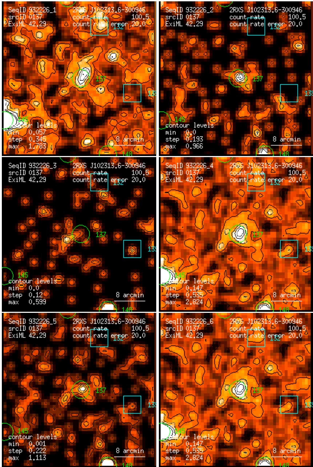
Figure 137: RASS 932226: detection 0137: band rate images, Gaussian filter: (1) PSPC channels 11 – 41, (2) 52 – 90, (3) 91 – 201, (4) 11 – 235, (5) 52 – 201, (6) 11 – 201. Broad band rates in counts/ks. Band rate contour levels in counts/ks/arcmin 2 .
