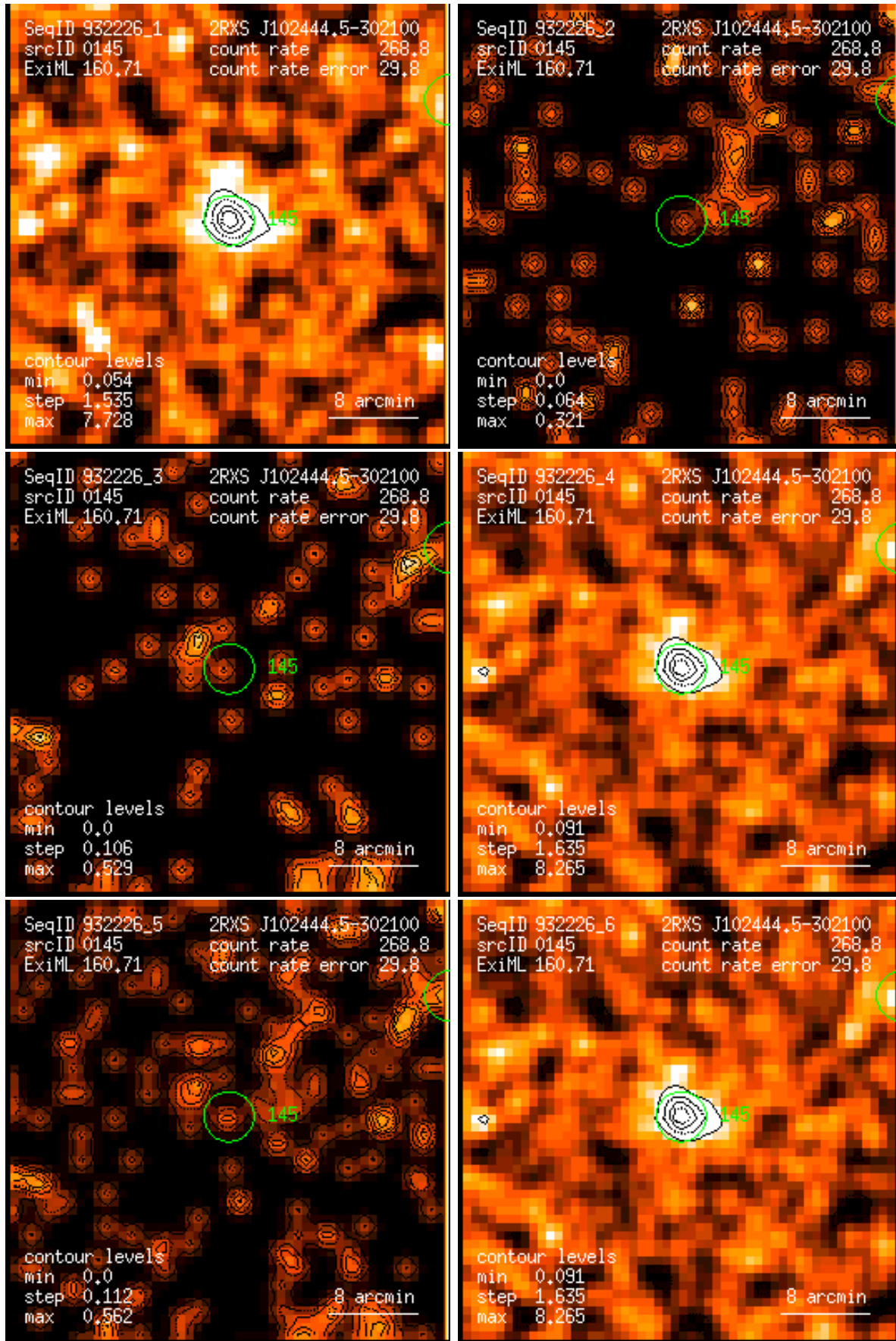
Figure 145: RASS 932226: detection 0145: band rate images, Gaussian filter: (1) PSPC channels 11 – 41, (2) 52 – 90, (3) 91 – 201, (4) 11 – 235, (5) 52 – 201, (6) 11 – 201. Broad band rates in counts/ks. Band rate contour levels in counts/ks/arcmin 2 .
