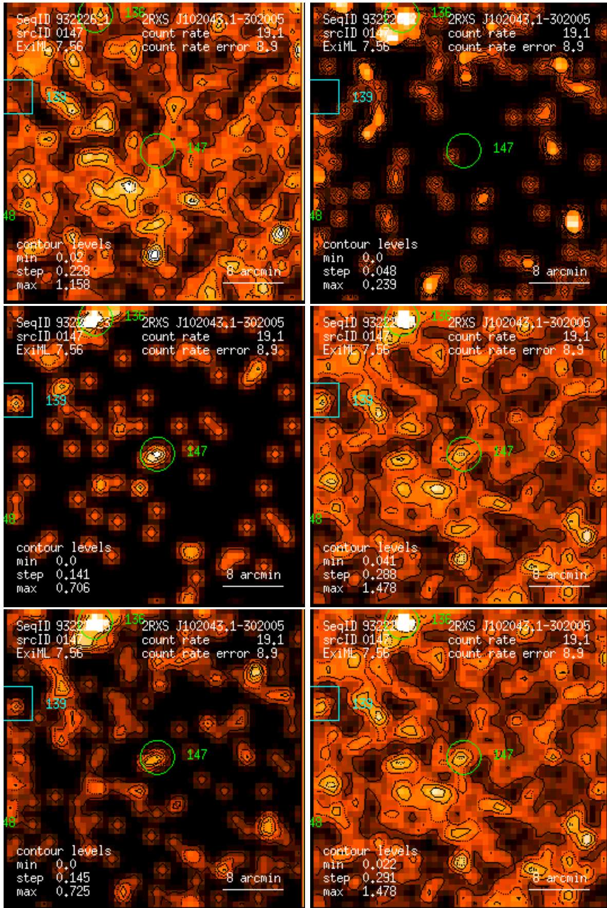
Figure 147: RASS 932226: detection 0147: band rate images, Gaussian filter: (1) PSPC channels 11 – 41, (2) 52 – 90, (3) 91 – 201, (4) 11 – 235, (5) 52 – 201, (6) 11 – 201. Broad band rates in counts/ks. Band rate contour levels in counts/ks/arcmin 2 .
