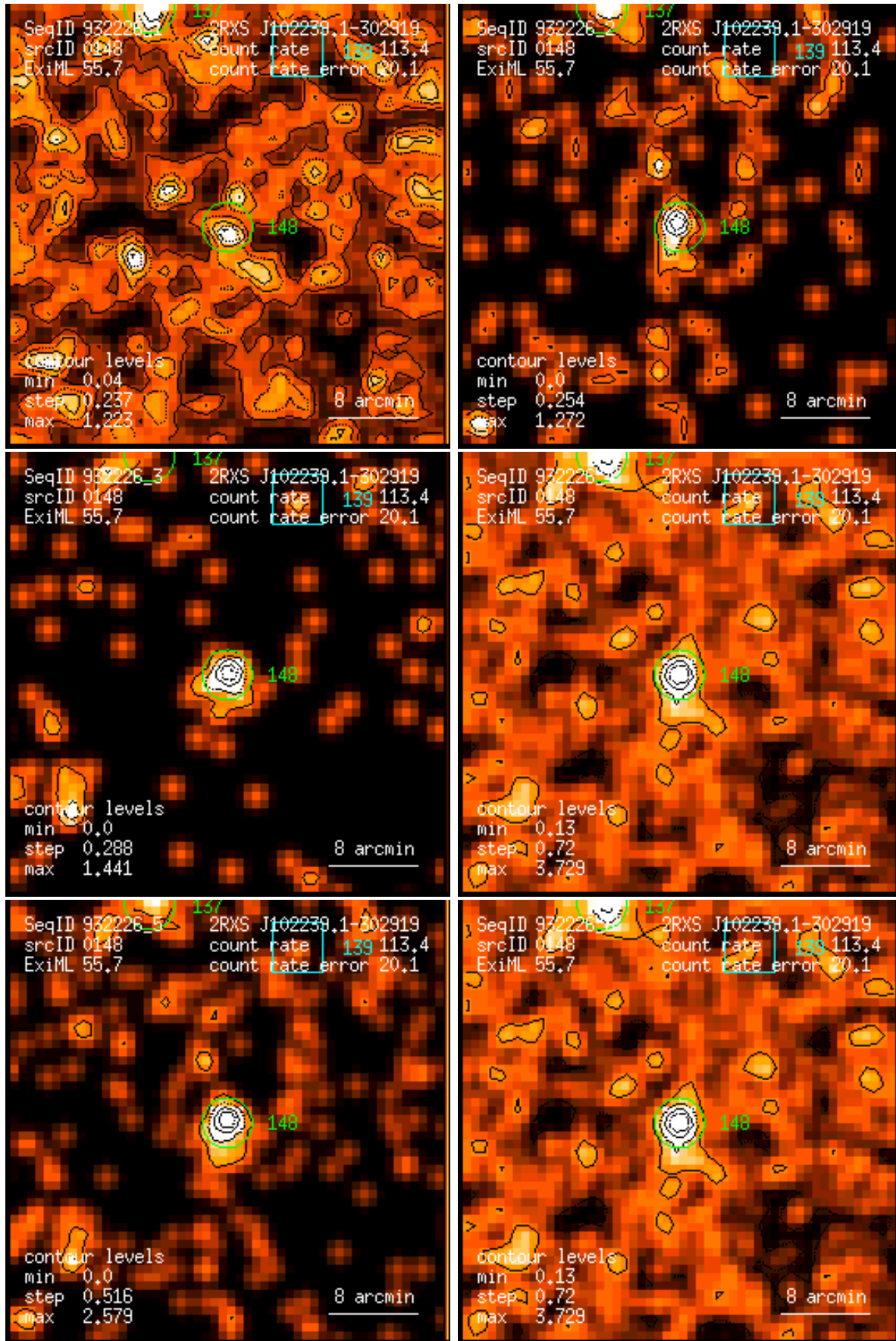
Figure 148: RASS 932226: detection 0148: band rate images, Gaussian filter: (1) PSPC channels 11 – 41, (2) 52 – 90, (3) 91 – 201, (4) 11 – 235, (5) 52 – 201, (6) 11 – 201. Broad band rates in counts/ks. Band rate contour levels in counts/ks/arcmin 2 .
