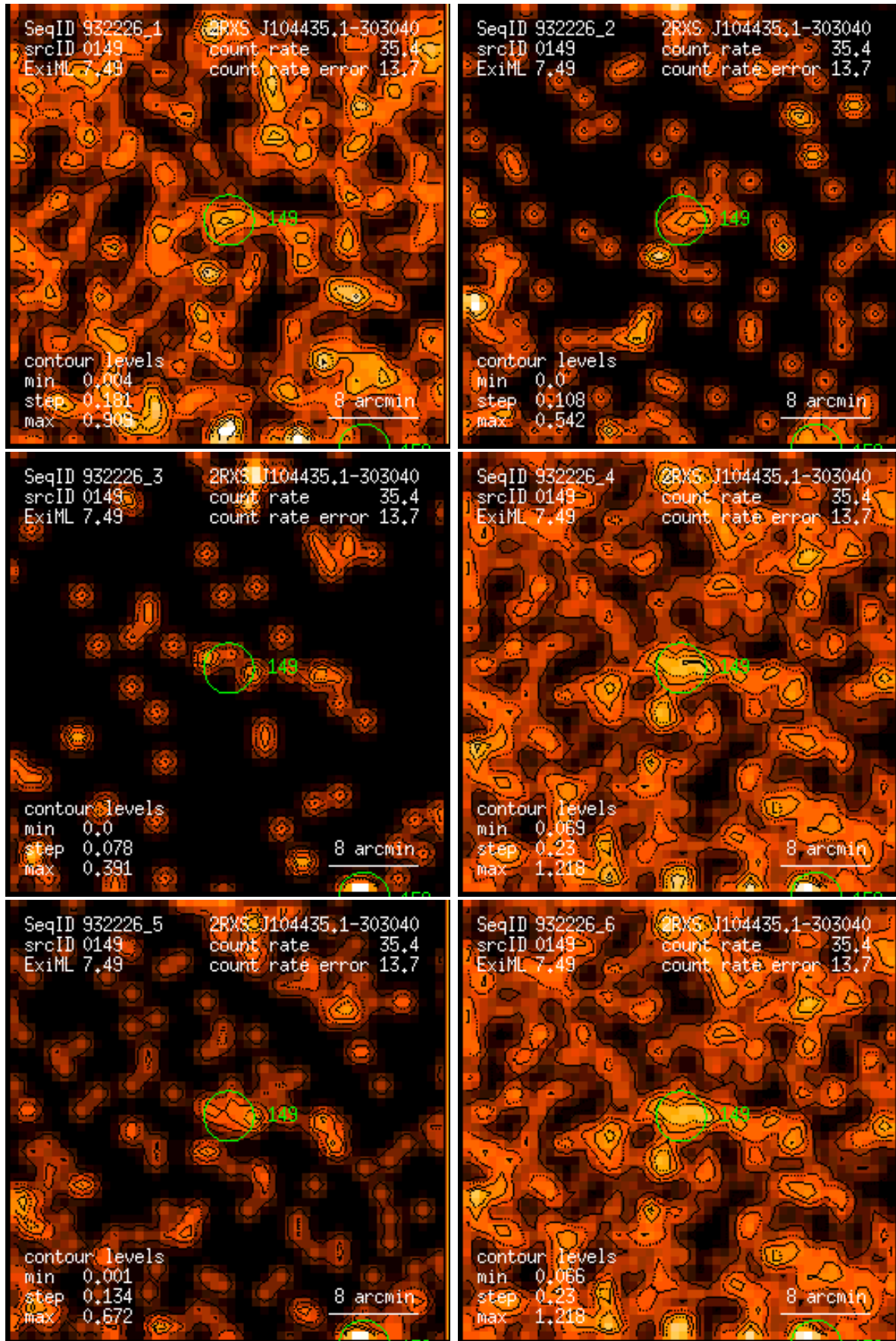
Figure 149: RASS 932226: detection 0149: band rate images, Gaussian filter: (1) PSPC channels 11 – 41, (2) 52 – 90, (3) 91 – 201, (4) 11 – 235, (5) 52 – 201, (6) 11 – 201. Broad band rates in counts/ks. Band rate contour levels in counts/ks/arcmin 2 .
