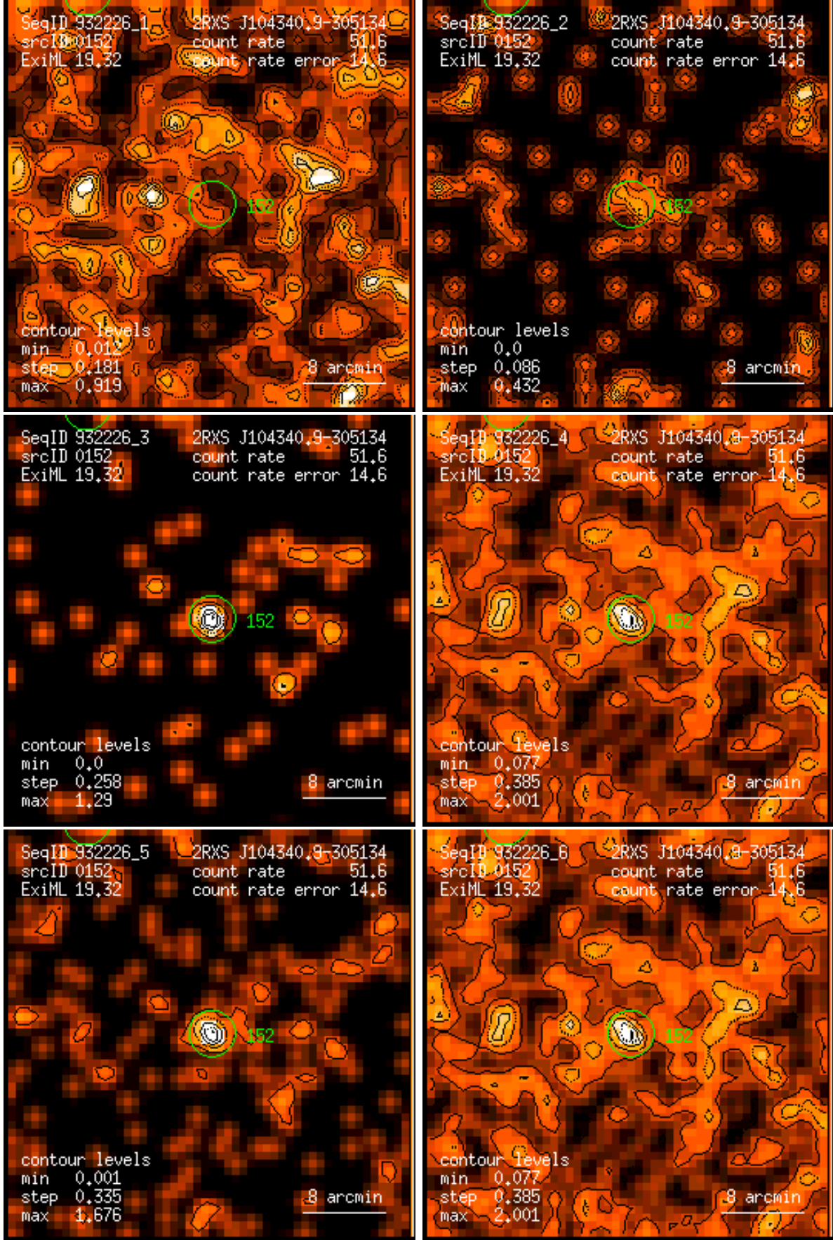
Figure 152: RASS 932226: detection 0152: band rate images, Gaussian filter: (1) PSPC channels 11 – 41, (2) 52 – 90, (3) 91 – 201, (4) 11 – 235, (5) 52 – 201, (6) 11 – 201. Broad band rates in counts/ks. Band rate contour levels in counts/ks/arcmin 2 .
