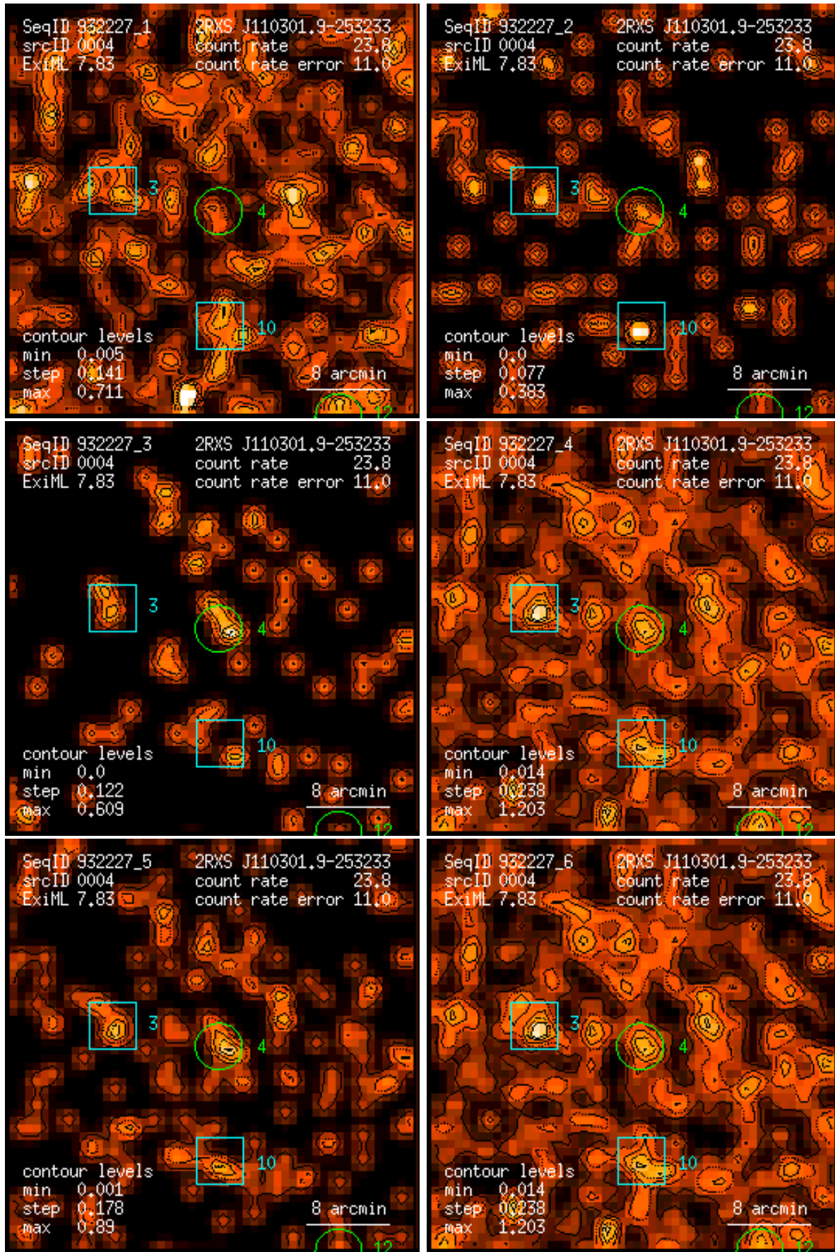
Figure 4: RASS 932227: detection 0004: band rate images, Gaussian filter: (1) PSPC channels 11 – 41, (2) 52 – 90, (3) 91 – 201, (4) 11 – 235, (5) 52 – 201, (6) 11 – 201. Broad band rates in counts/ks. Band rate contour levels in counts/ks/arcmin 2 .
